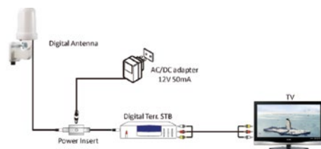
Installation : Connected Through Power Supply Kits (Fig.1)
