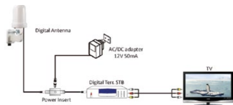
Installation : Connected Through Power Supply Kits (Fig.1)
