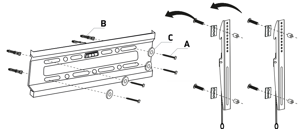
(A) M6x50 Self-tapping screw (4)
