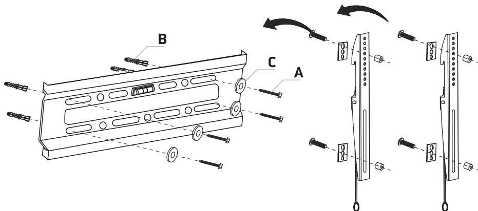
(A) M6x50 Self-tapping screw (4)
