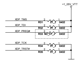
PU/PD for JTAG signals
