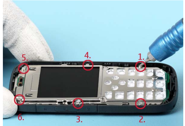
6) Unscrew the 6ea. #4 TORX screws in the order shown.
