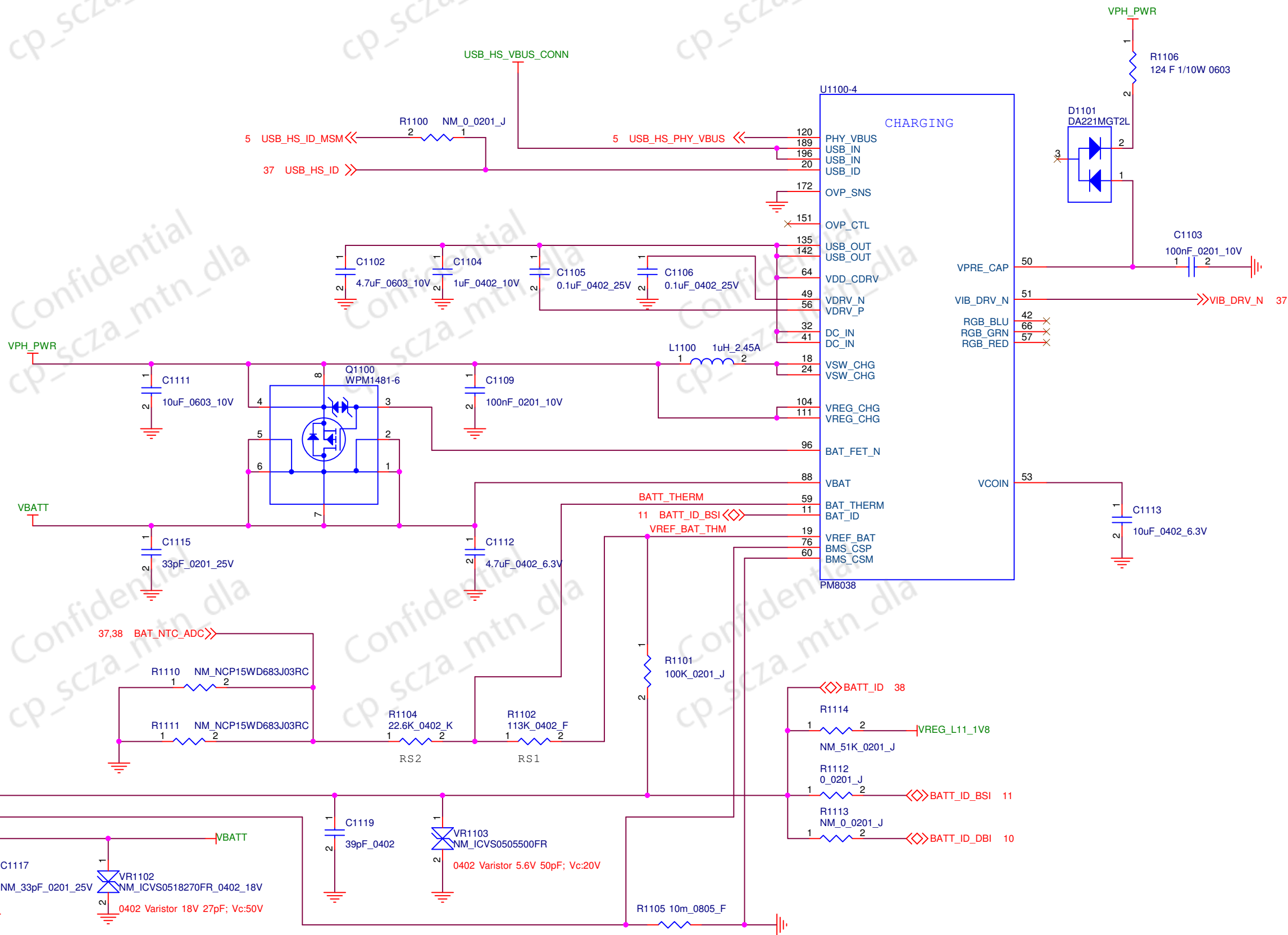
PM8038 Charging/Gasgauge
