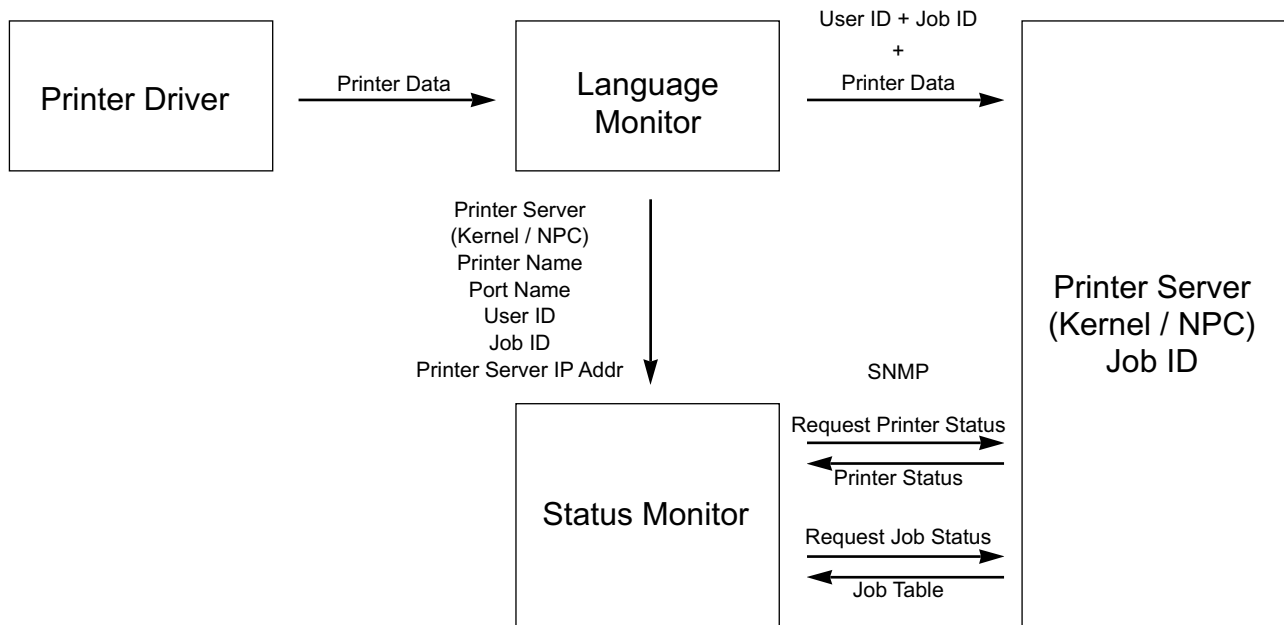
Status Monitor Data Flow
