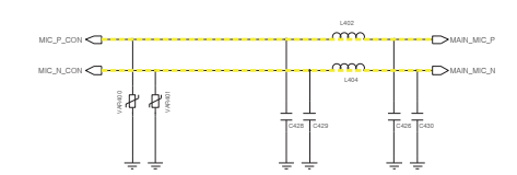
Main MIC
