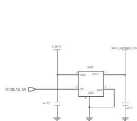
MIC BIAS LDO
