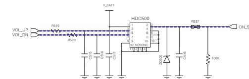
POWER & VOLUME KEY
