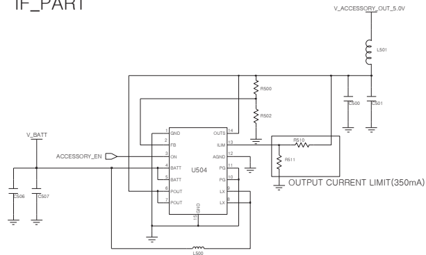
ACCESSORY_PWR
