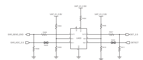
Comparator
