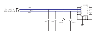
Left SPK conn
