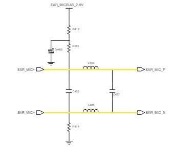
Ear MIC
