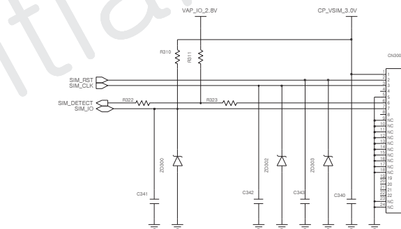
SIM Connector
