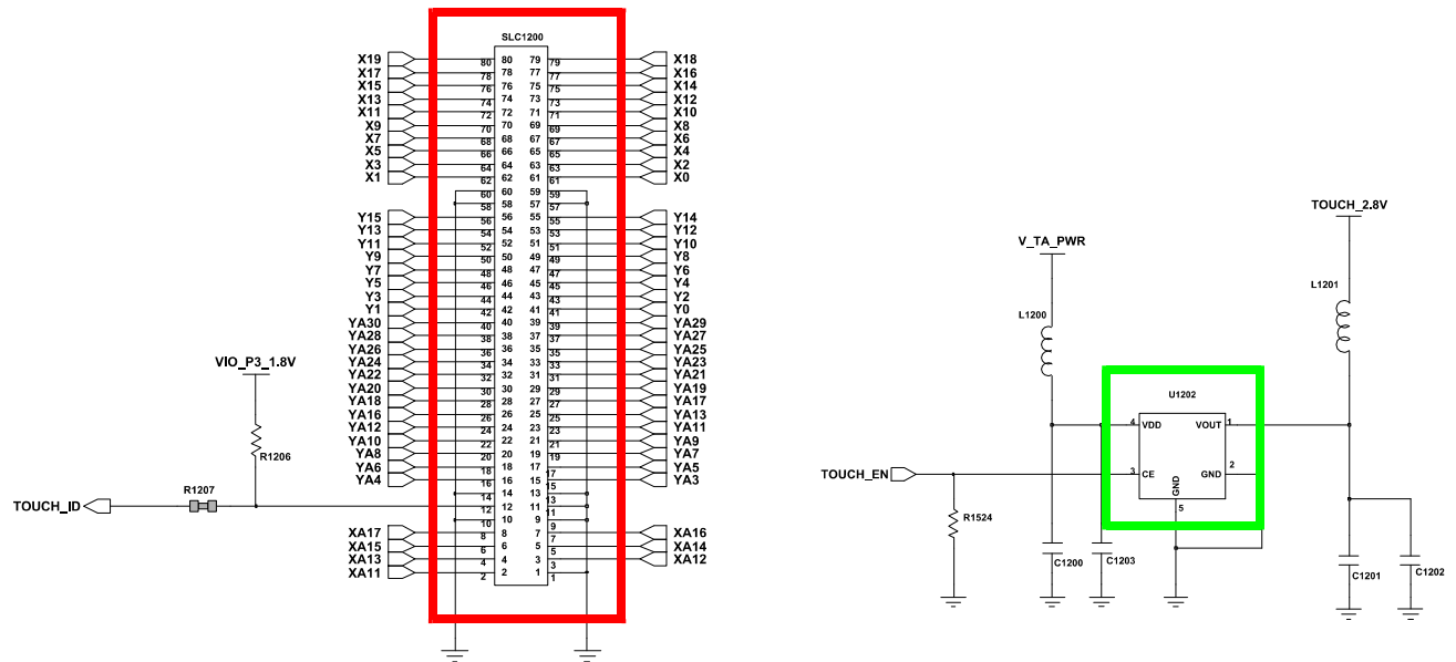
<80Pin TOUCH Con.>
