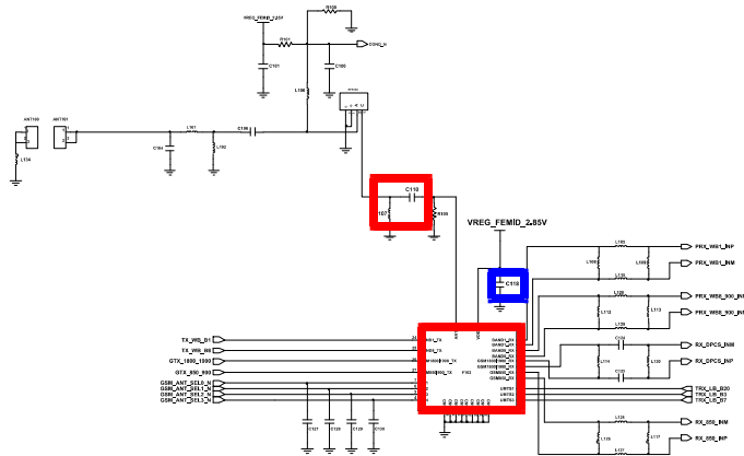
SWITCH(MAIN)
