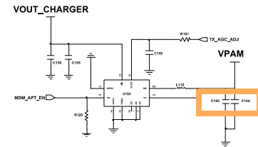
SMPS for VPAM
