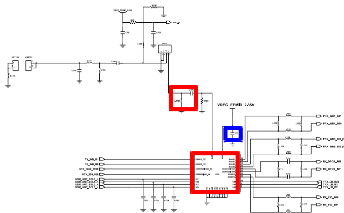
SWITCH(MAIN)
