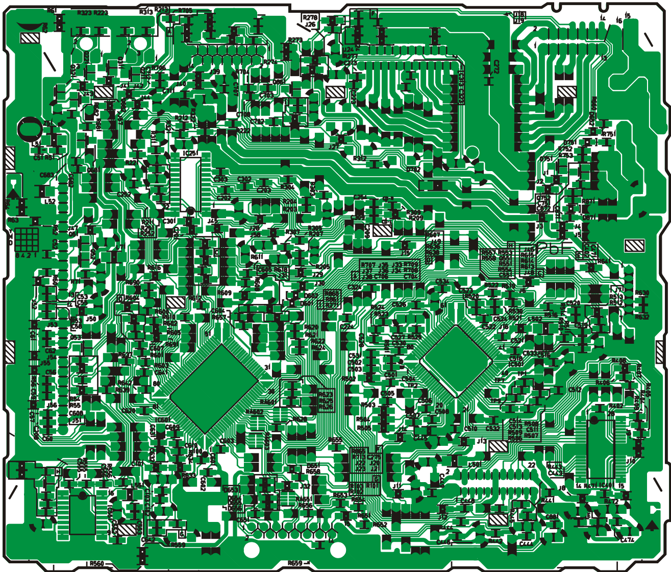
[E-4C312][BOTTOM VIEW]
