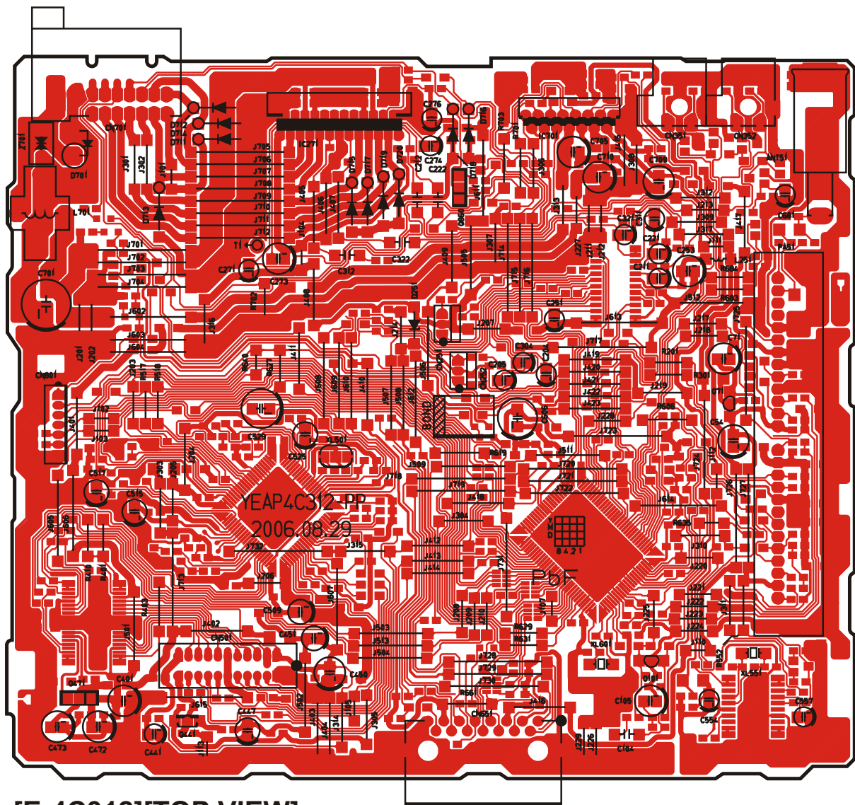
[E-4C312][TOP VIEW]
