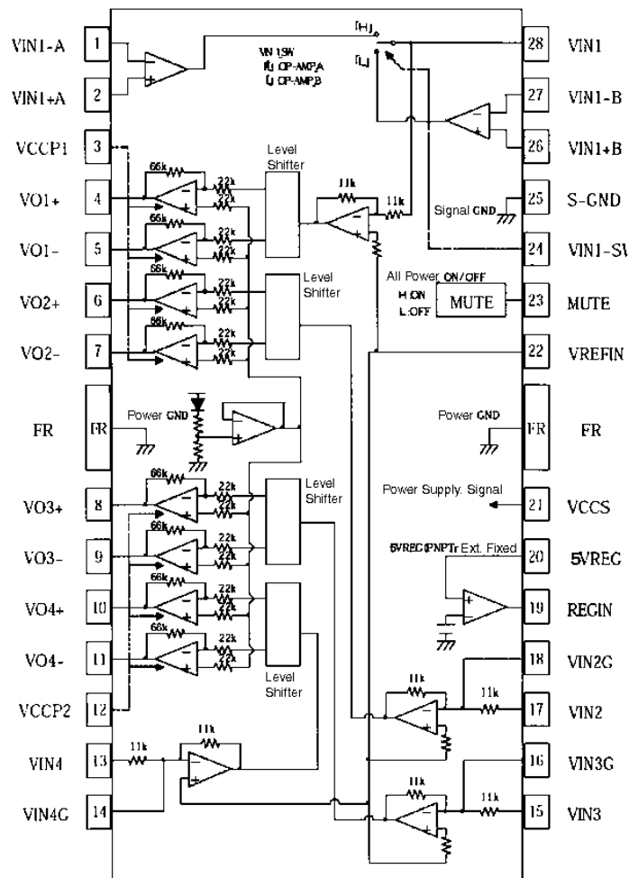
IC401 : C1BB00001088
