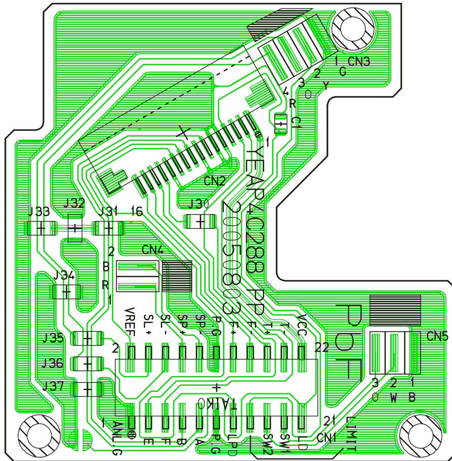
[E-4C288][BOTTOM VIEW]
