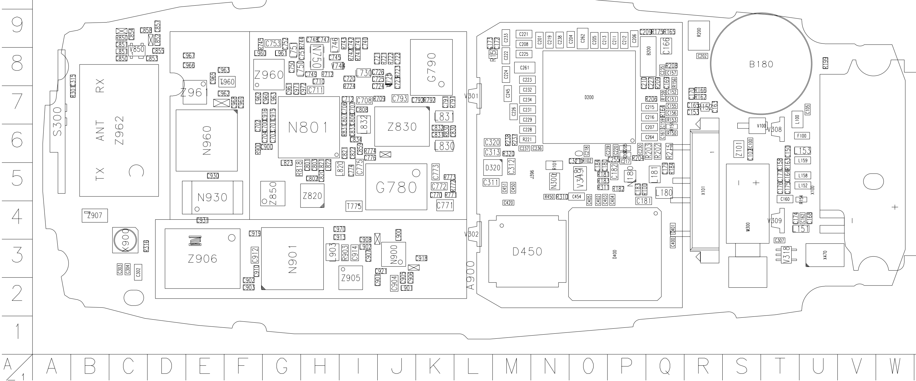
Component Layout Diagram 3560 - Top
