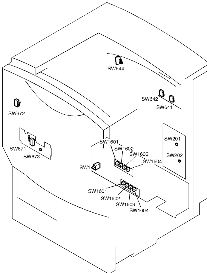
Figure 61. Printer switches
