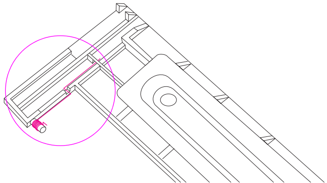
Figure 89. Spring on right cover subassembly
