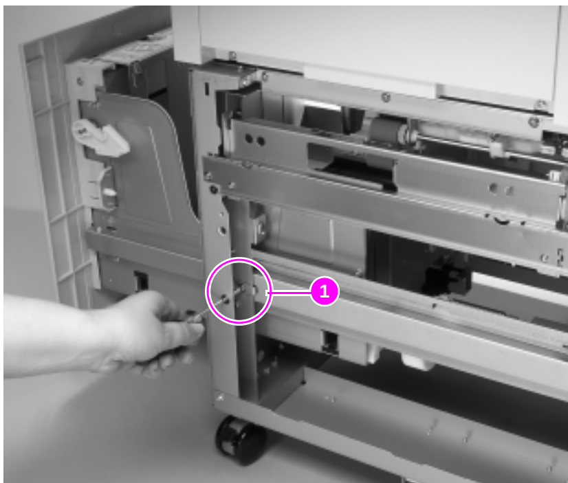
Figure 146. Tray 4 removal
