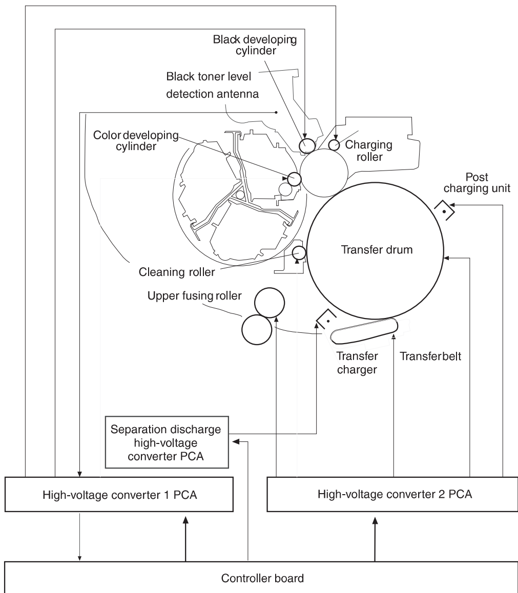
Figure 49. High-voltage power supply circuit
