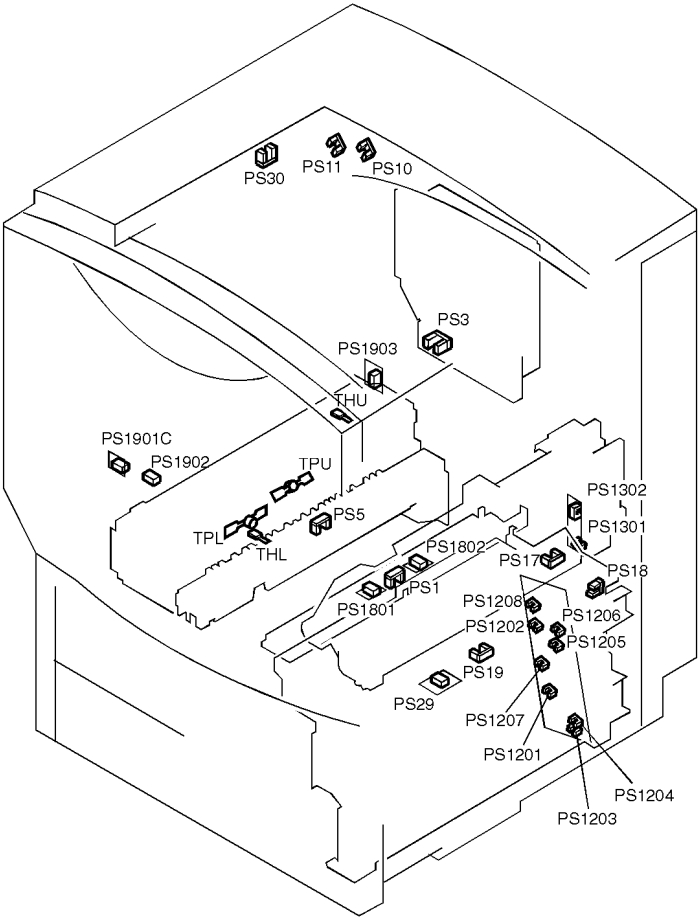
Figure 60. Printer sensors
