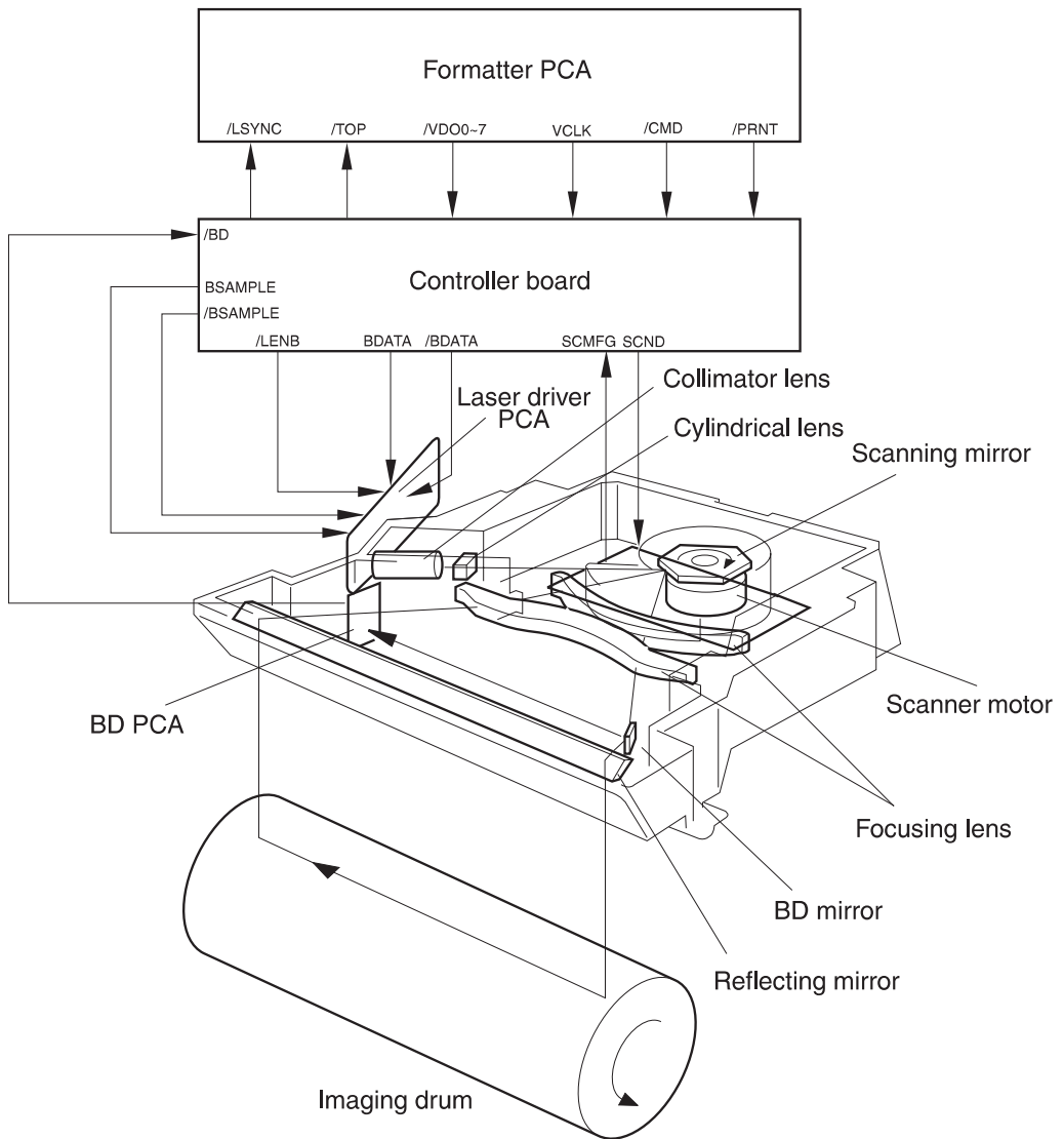
Figure 50. Laser/scanner
