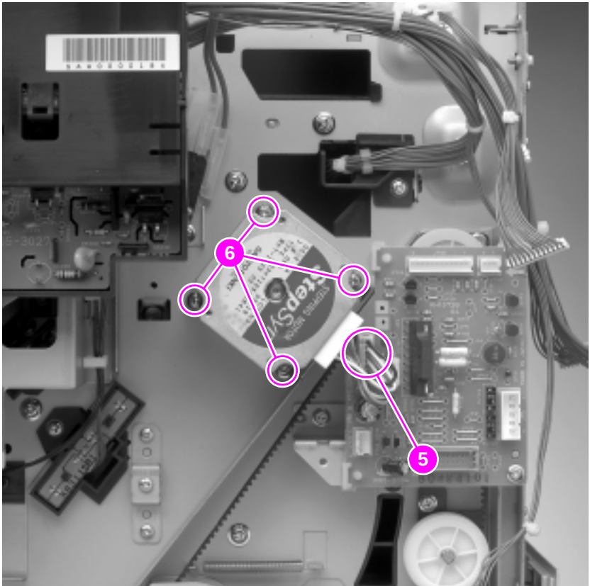
Figure 128. Carousel motor
