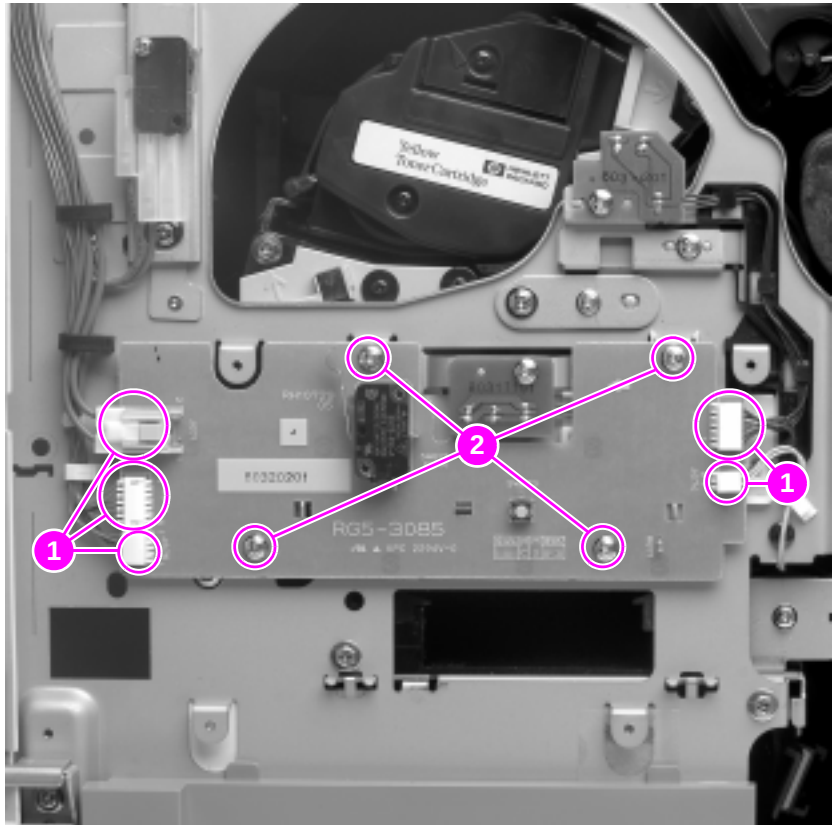
Figure 99. Subrelay PCA
