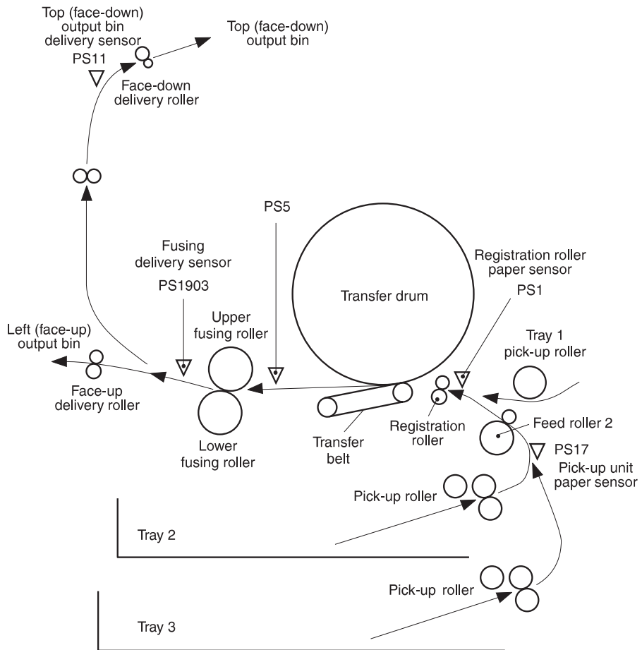
Figure 57. Paper path
