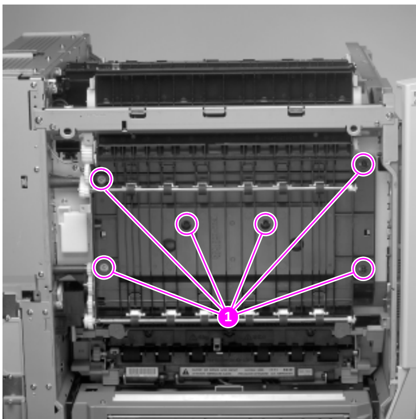
Figure 103. Feeder assembly
