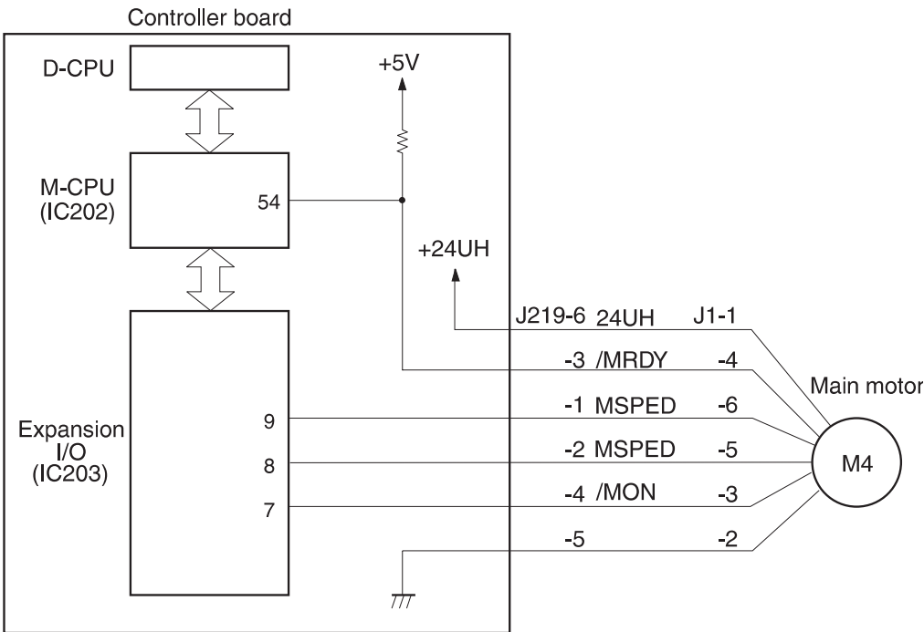
Figure 55. Main motor (M4)
