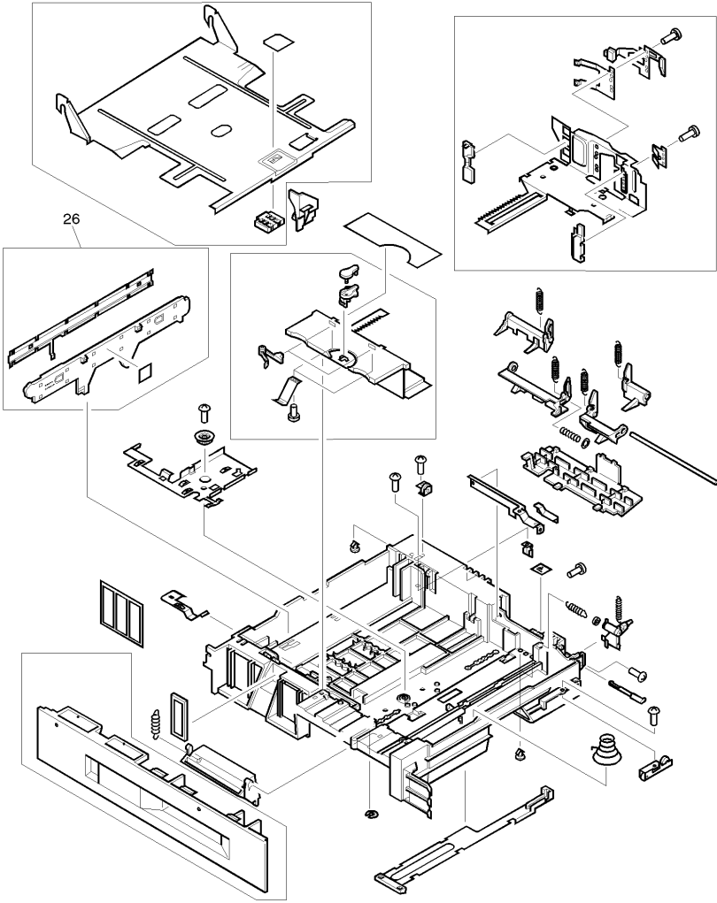
Figure 227. Tray 2 assembly
