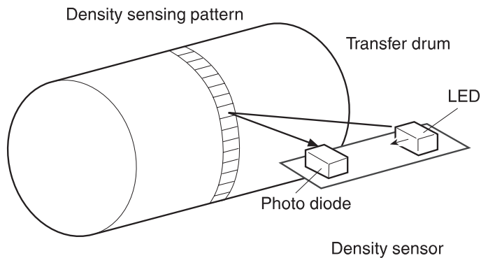
Figure 43. Density sensor
