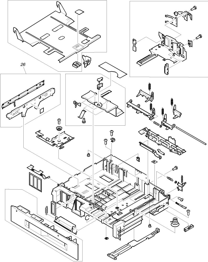
Figure 226. Tray 3 assembly
