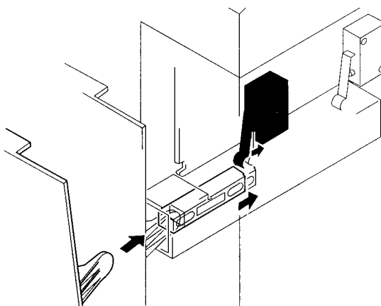
Figure 182. Right upper cover detection interlock
