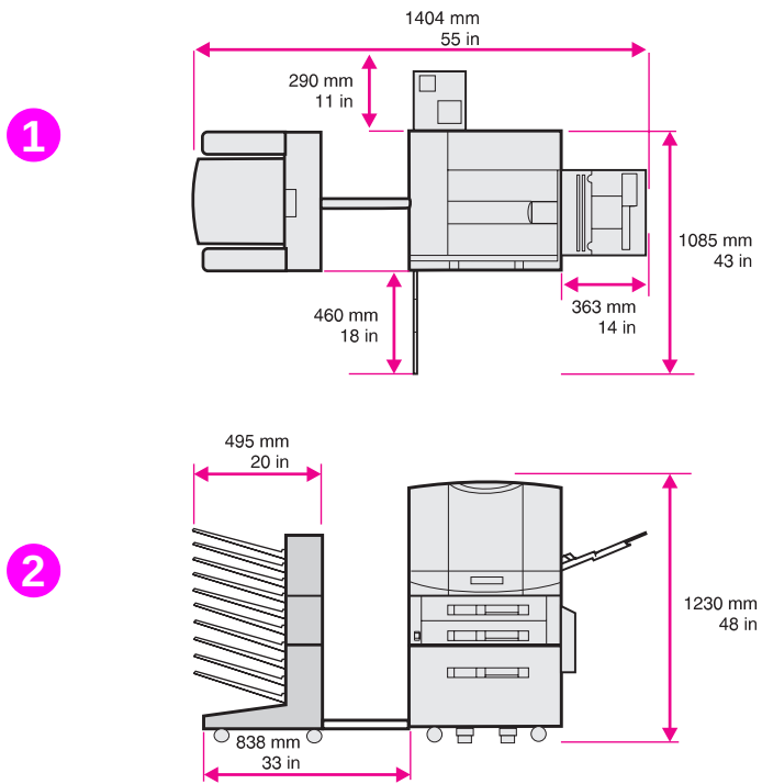
Figure 1. Space requirements
