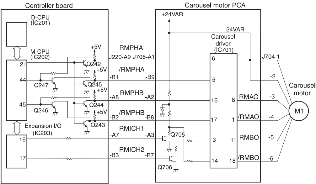
Figure 52. Carousel motor (M1)
