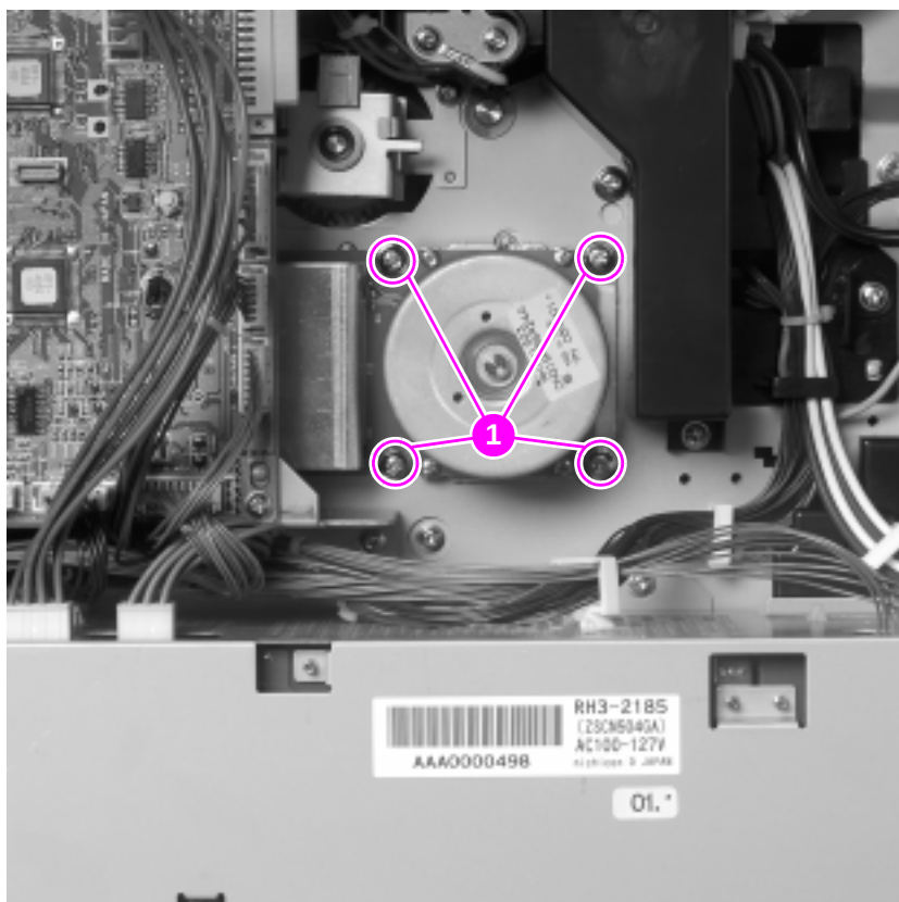
Figure 125. Main motor
