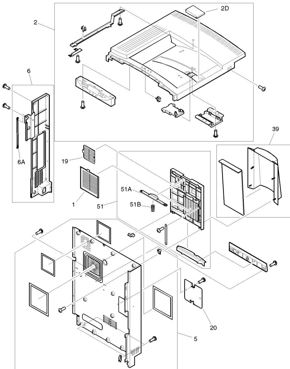
Figure 215. Printer covers and doors (2 of 3)
