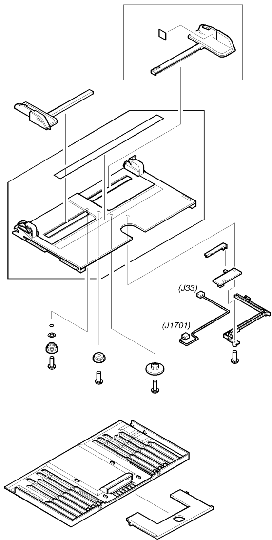
Figure 235. Tray 1 assembly
