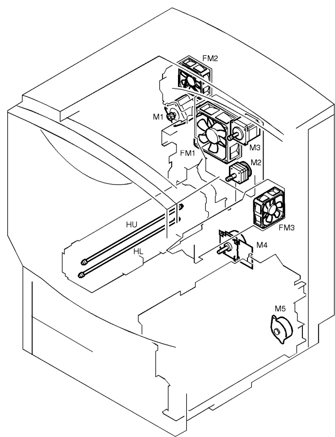
Figure 51. Printer motors and heaters
