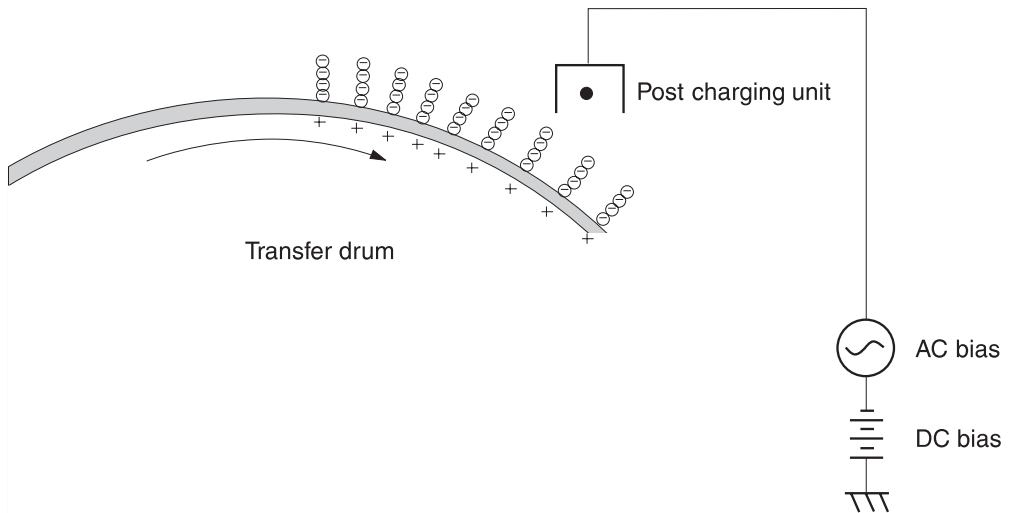
Figure 33. Post charging
