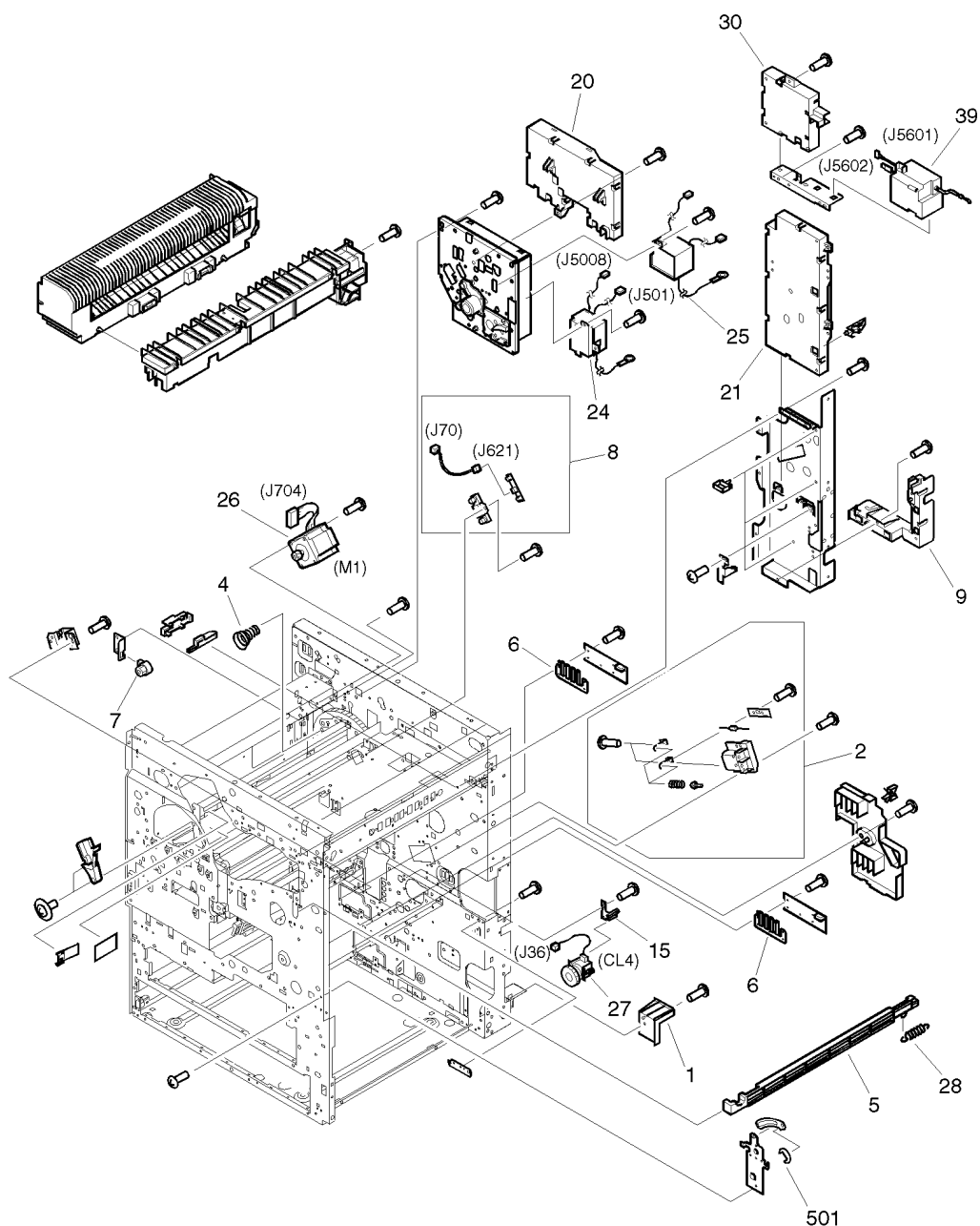
Figure 220. Internal components (3 of 6)
