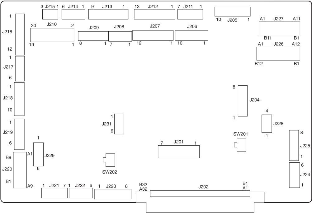
Figure 209. Connectors on the controller board
