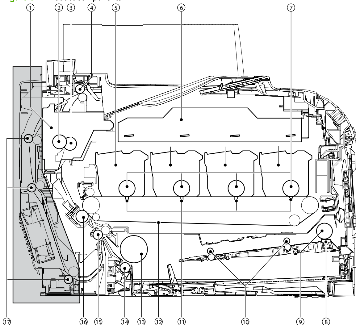
Figure 5-2 Product components
