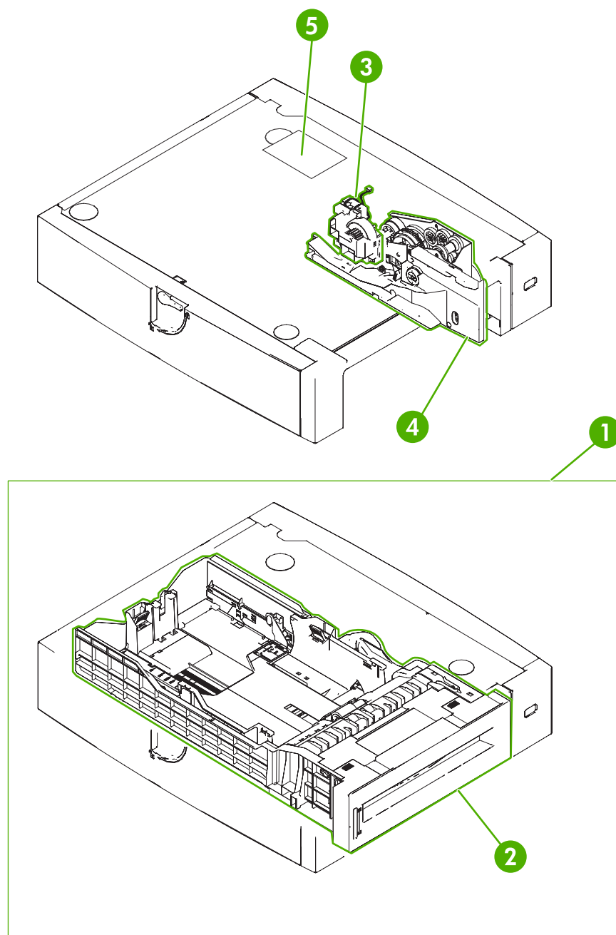
Figure 8-22 500-sheet paper feeder assembly
