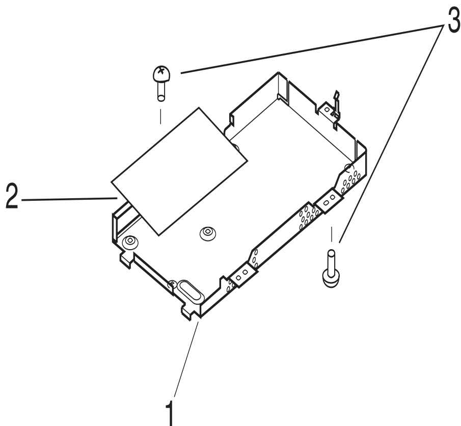
Figure 6-9 Formatter pan
