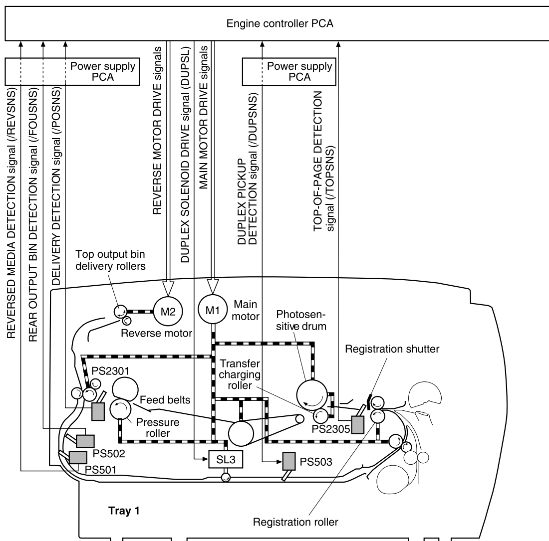
Figure 32. Automatic duplexer feed and delivery
