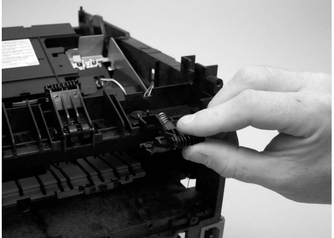
Figure 96. Removing the top-output-bin delivery assembly (3 of 3)
