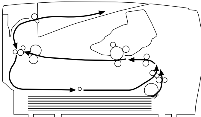
Figure 31. Automatic duplexer path
