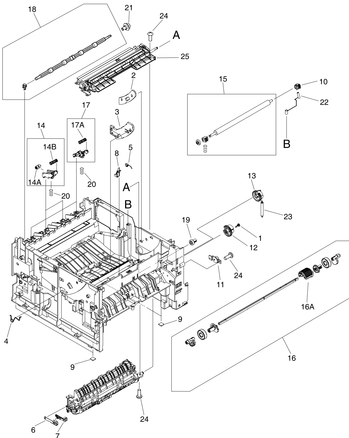
Figure 126. Internal components (2 of 4)
