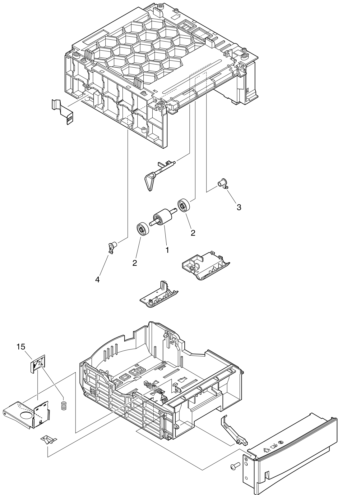
Figure 134. 500-sheet feeder
