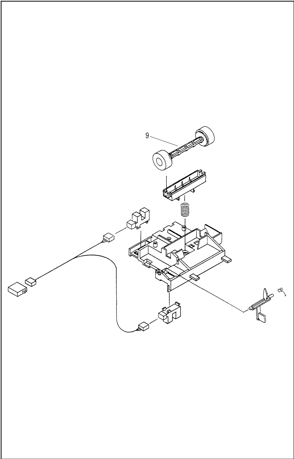
Feed Assembly
