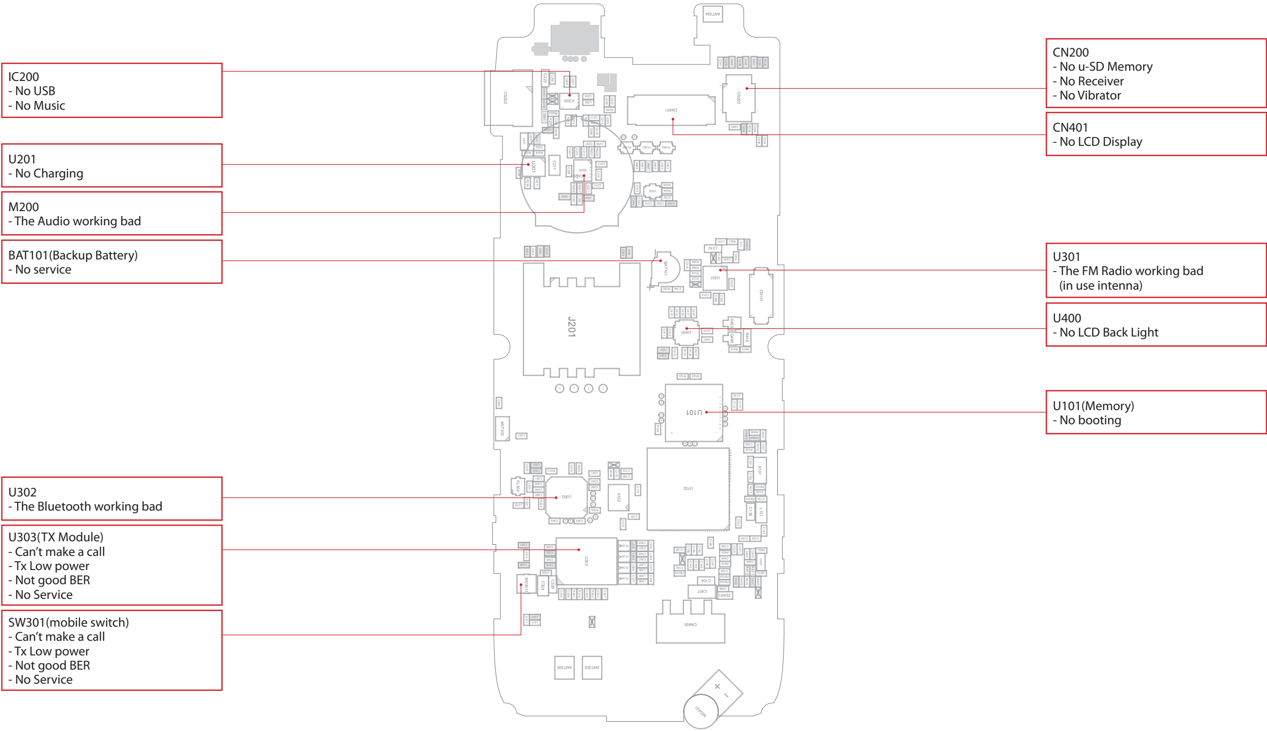
LG-A155_MAIN_SPFY0236101-1.0_BOT
