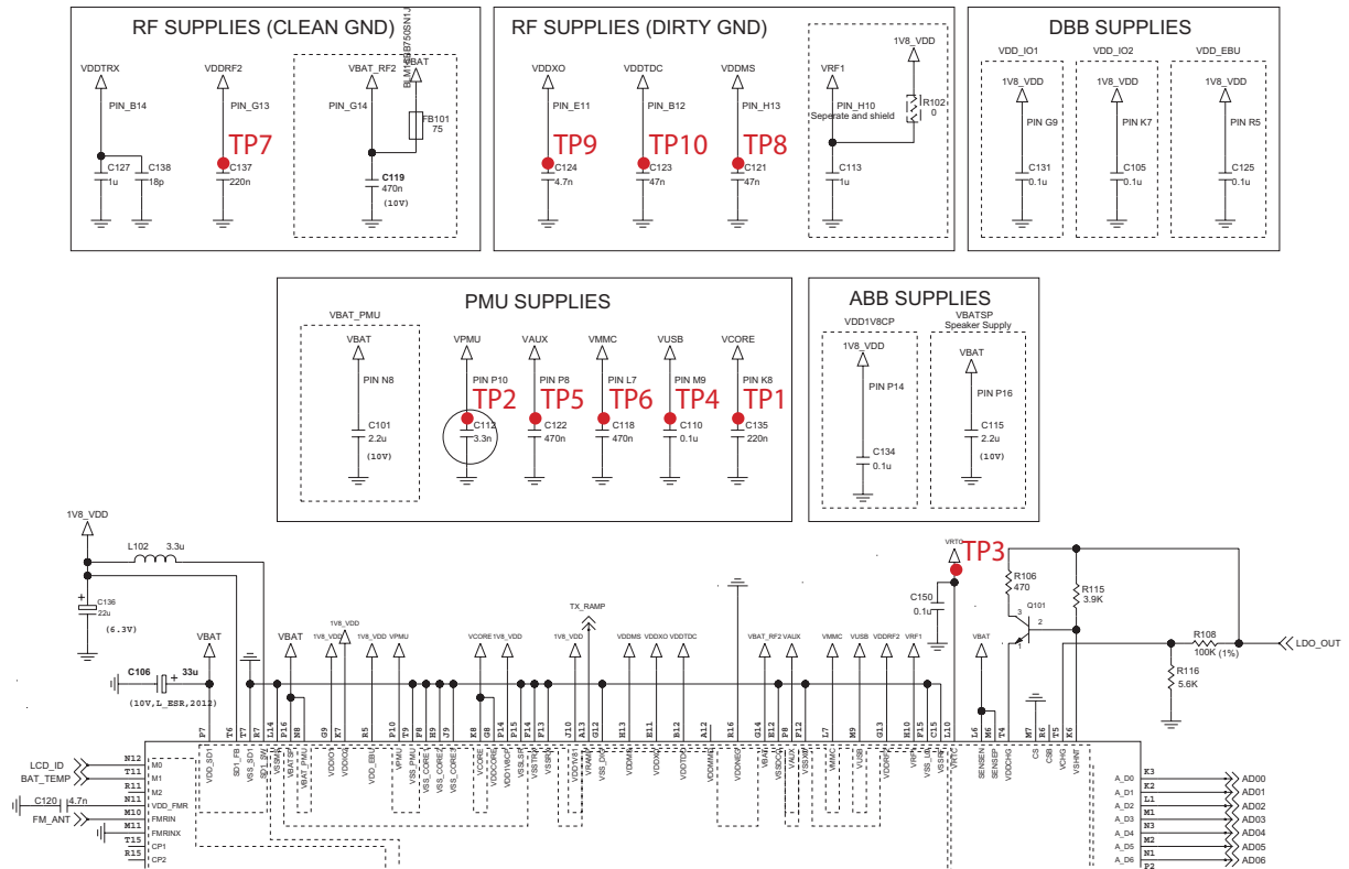
Figure 4.2 Power block of LG-A130
