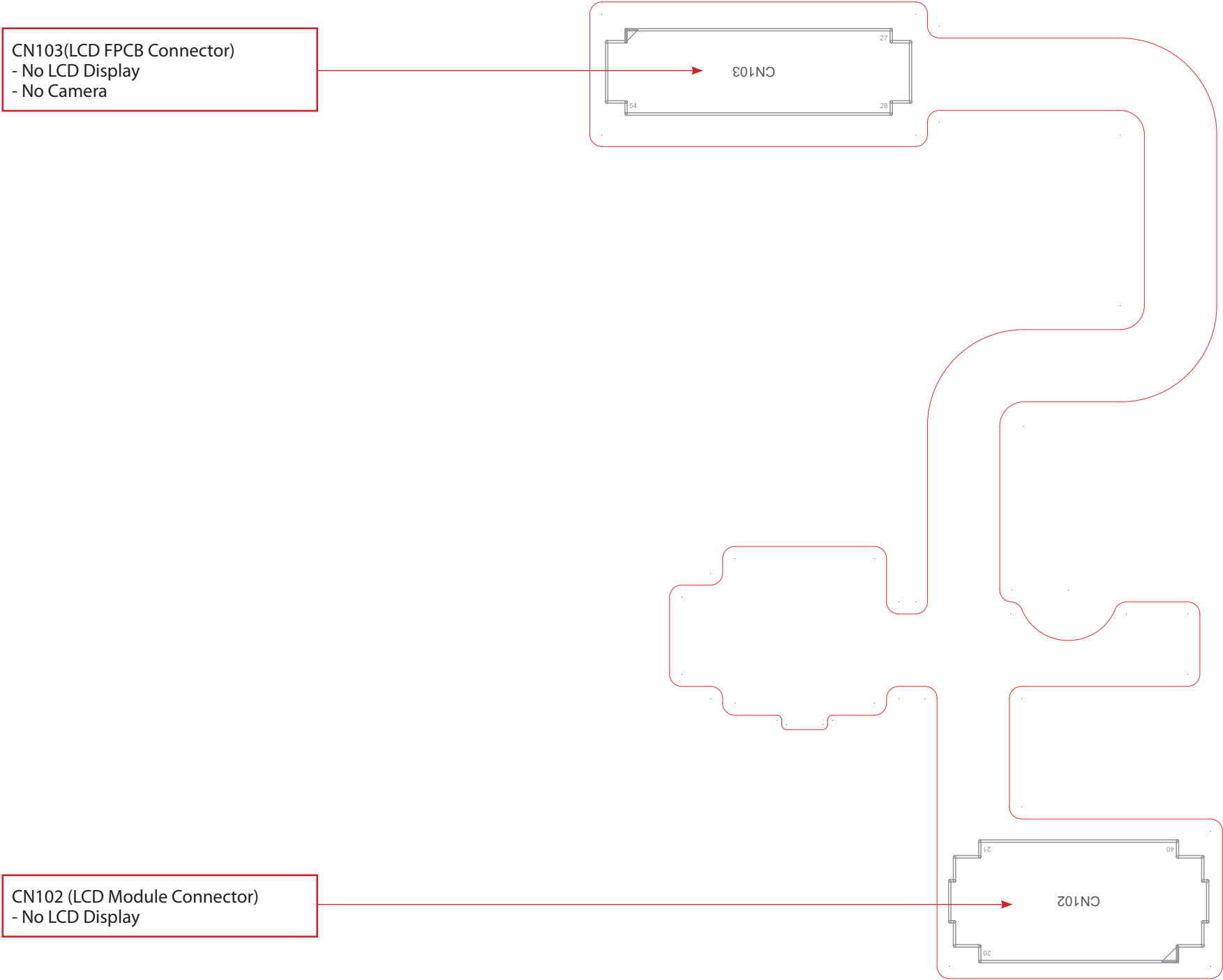
LG-A130_F_LCD_SPCY0232601-1.0
