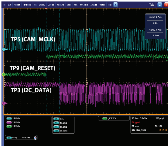
Graph 4.8.1. I2C Data Waveform
