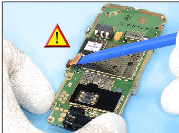
12. Carefully open the LCD connector with the SS-93. Take special care to the surrounding components.
