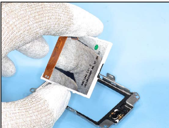
18. The LCD can be removed easily if both hooks are unlocked correctly.
