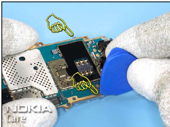
15. Unlock both clips of the KEYMAT LIGHT GUIDE ASSY. Bear in mind that these plastic clips are delicate and can break easily.
