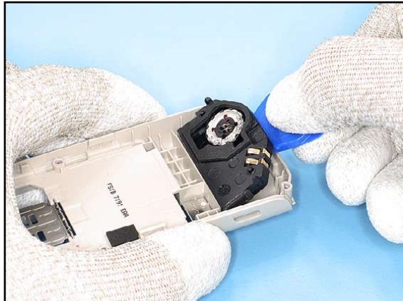
10. Pry out the ANTENNA MODULE with the SRT-6.
