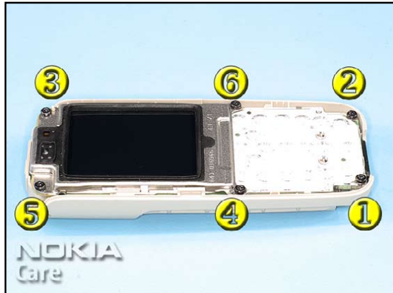
8. Undo the 6 Torx Plus size 6 screws in the order shown and remove them.
