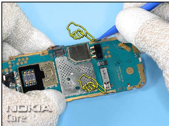
13. Unlock both clips of the UI SHIELD with the SS-93.
