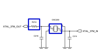
BT / WIFI XTAL ( 37.4 MHz )
