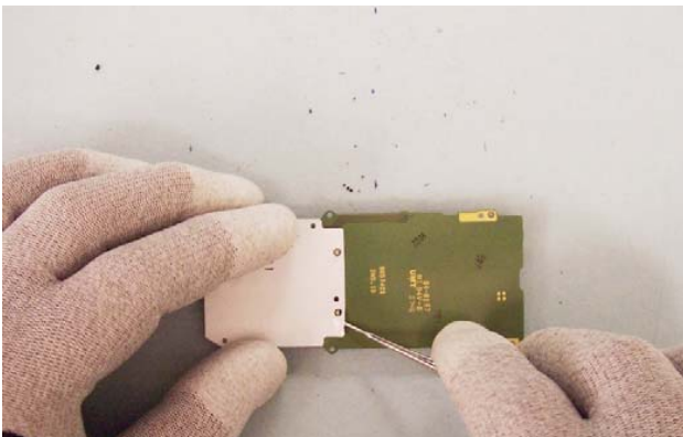
17) Use Pick to lift the Dome Sheet.
