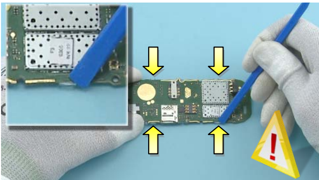
15) Use the SS-93 to release the four shown clips holding the LIGHT GUIDE. Be careful not to damage any nearby components.
