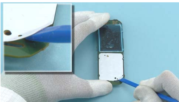
17) Peel off one corner of the DOMESHEET with the SS-93.
