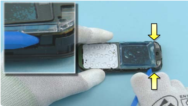
13) Lift up the ENGINE BOARD from the top side by releasing the two shown clips with the sharp end of the SS-93.
