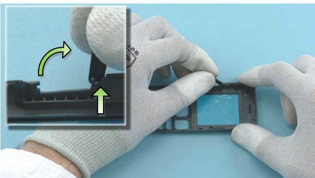
23) Flip open and remove the SD DOOR.
