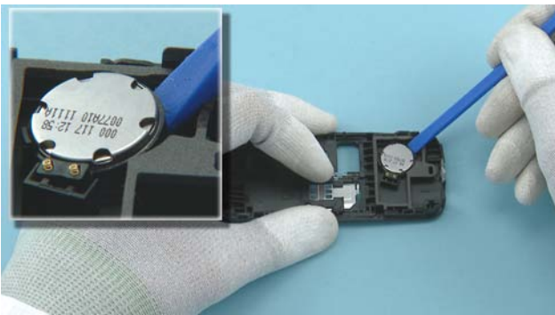
21) Lift up the EARPIECE/SPEAKER/VIBRA with the SS-93.
