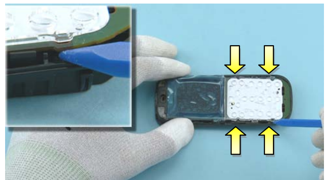
12) Lift the ENGINE BOARD up from the bottom side by releasing the four shown clips with the sharp end of the SS-93.
