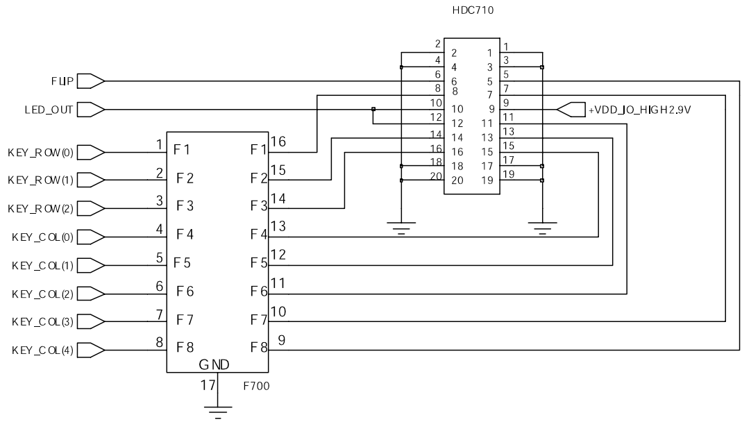
KEY_C ONNECTOR
