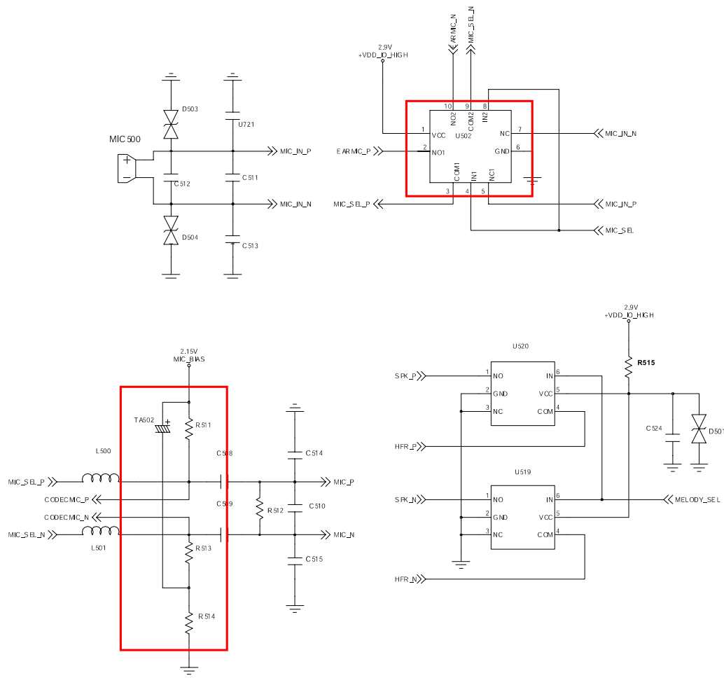
MICROPHONE
