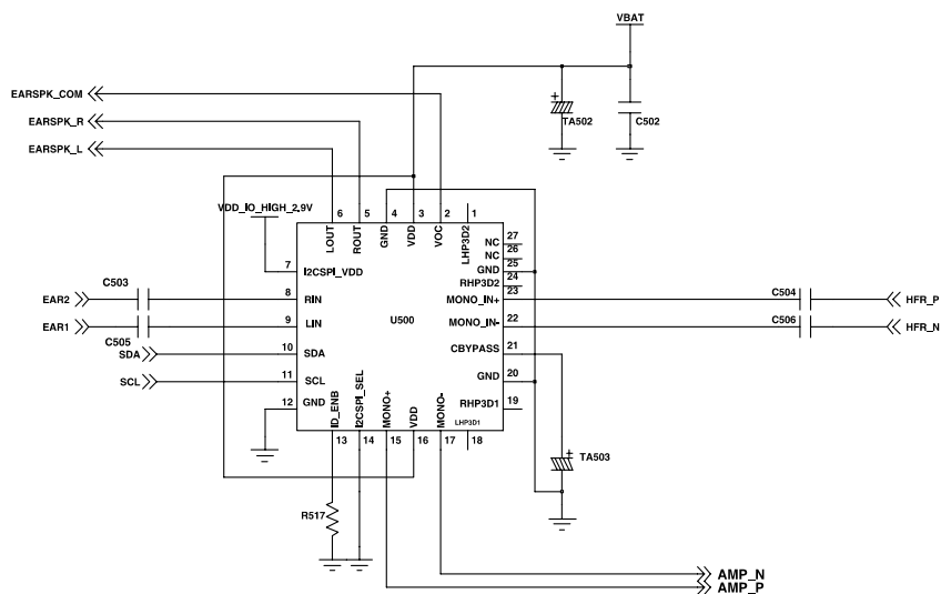
AUDIO AMP
