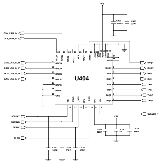
TRANSMITTER & RECEIVER
