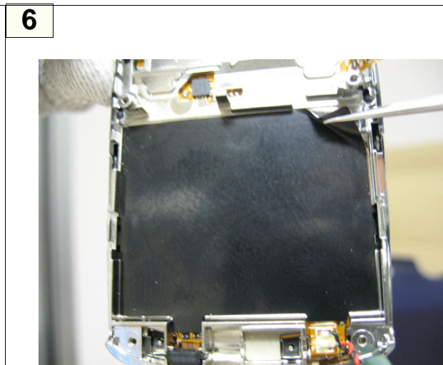
1) Remove The Black film from FRONT.
