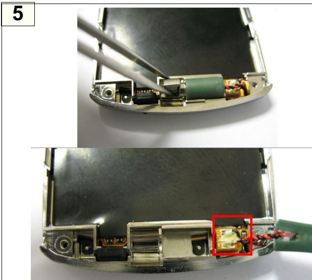
1) Disassemble the MOTOR from the FRONT.
