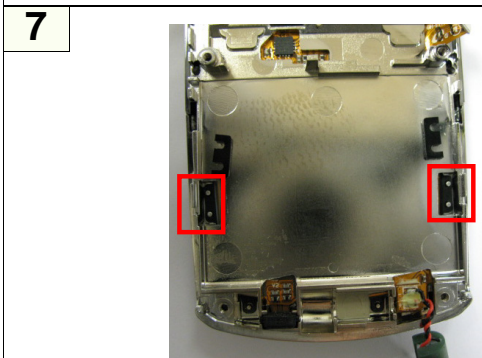
1) Remove rubbers in 2 flange position.
