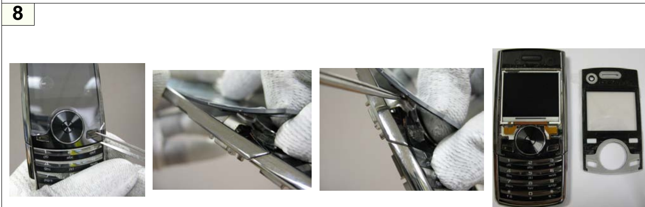
1) Remove rubbers in 2 flange position.
