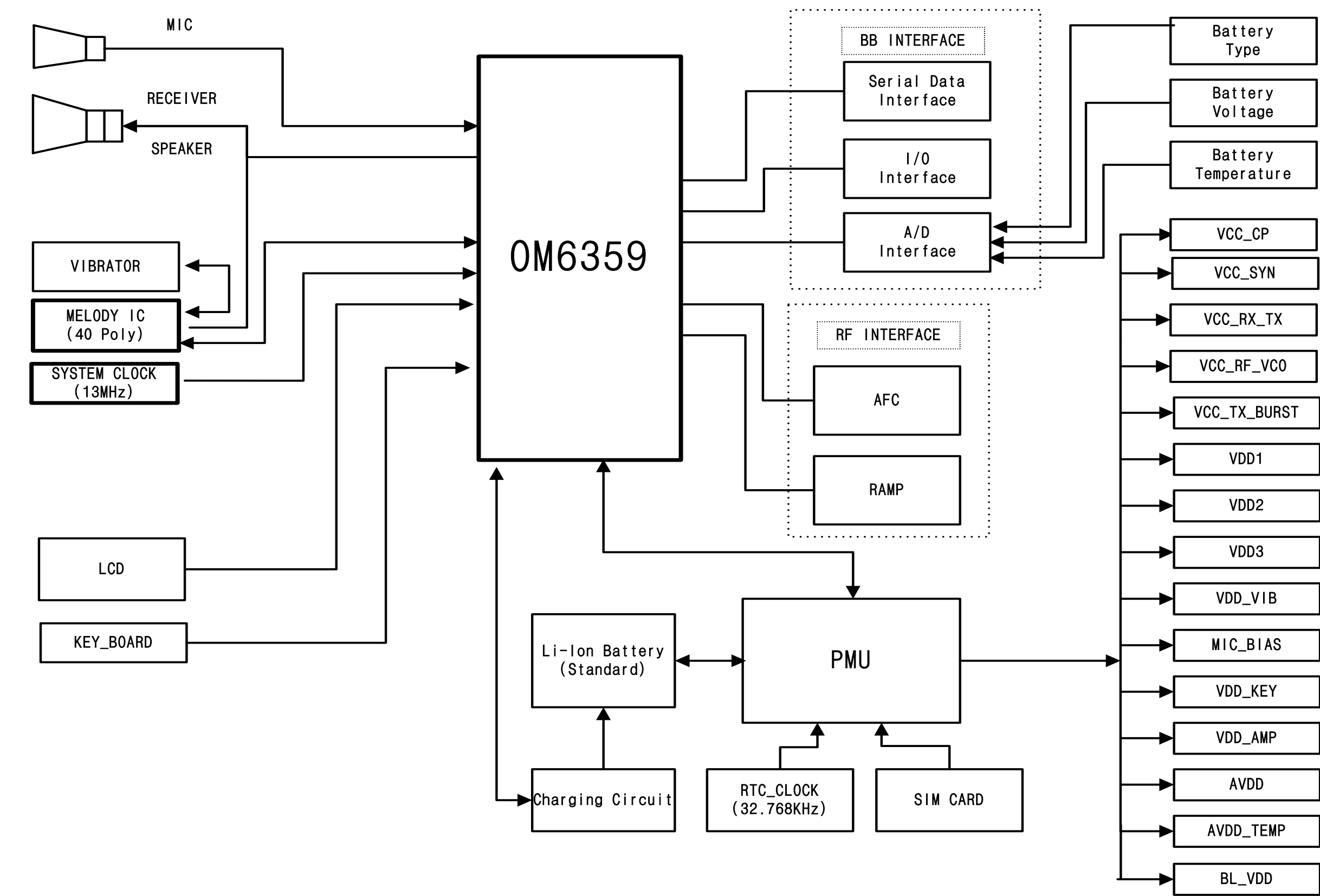
5-2. Base Band Solution Block Diagram
