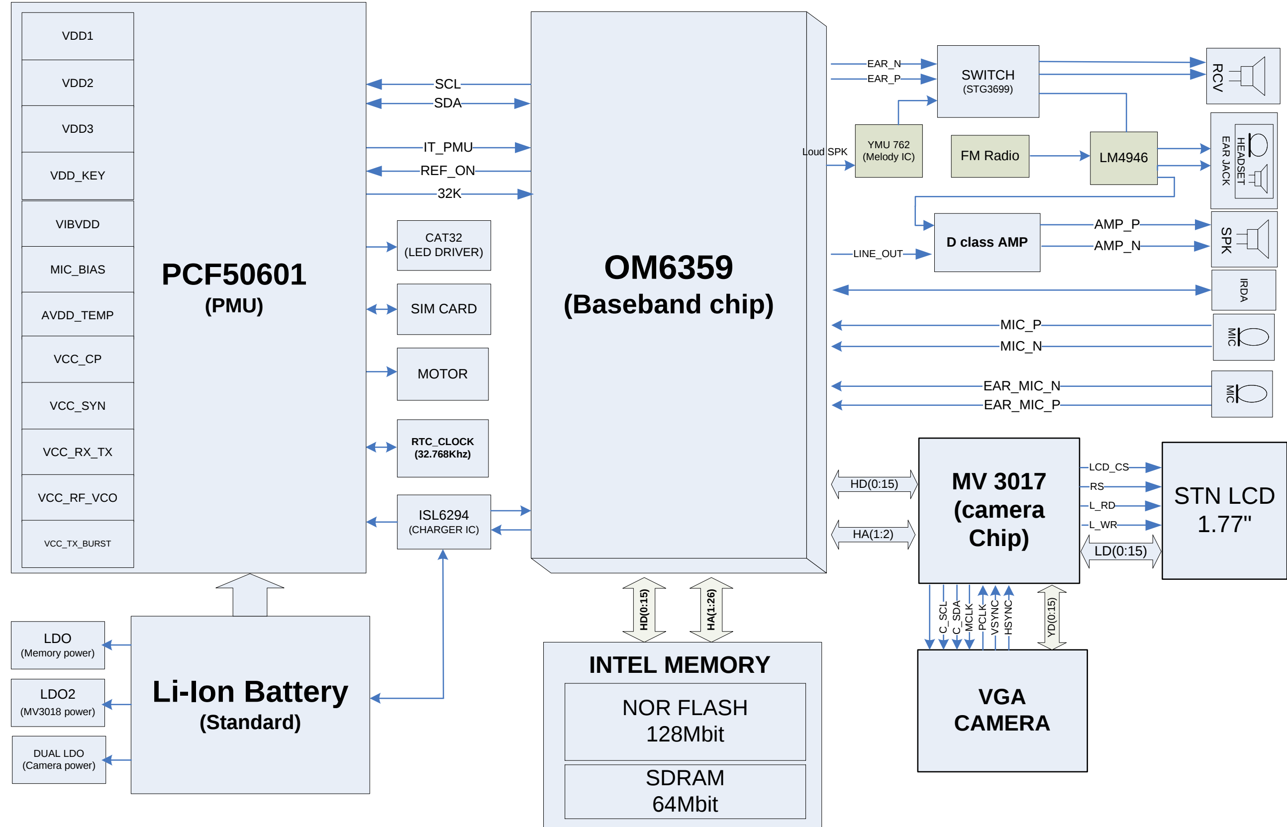
5-2. Base Band Solution Block Diagram
