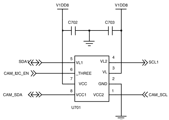
<CAM LEVEL TRANSLATOR>
