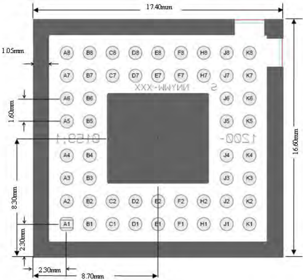
TOP VIEW
