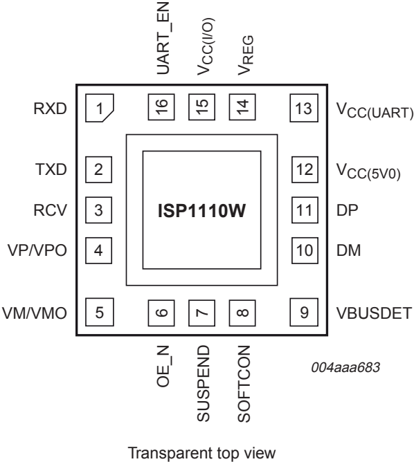
Pin configuration HBCC16; top view.
