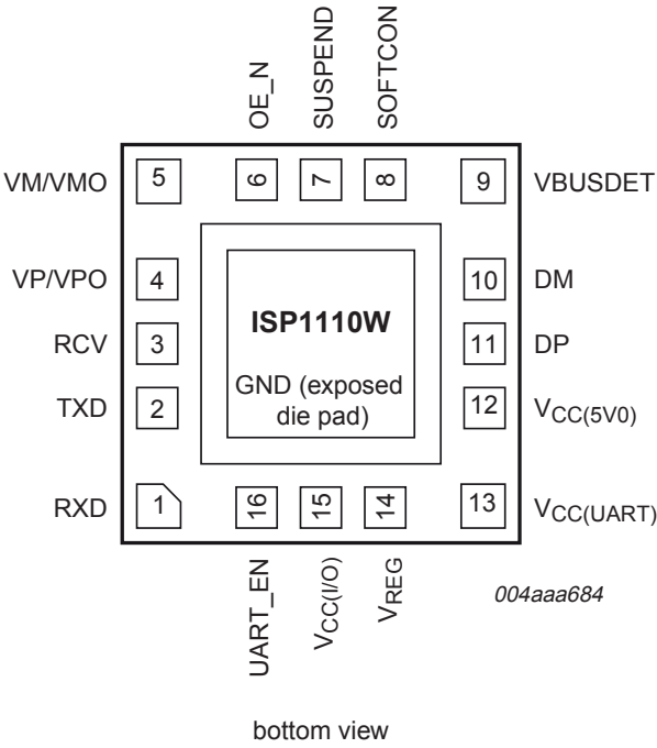
Pin configuration HBCC16; bottom view.
