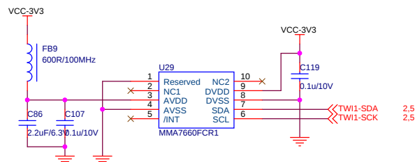
G-sensor
