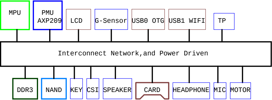
BLOCK
