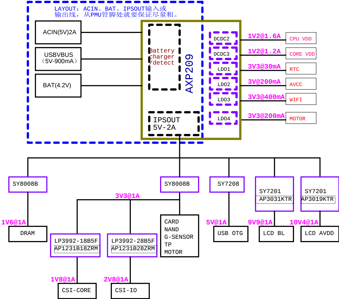
POWER TREE
