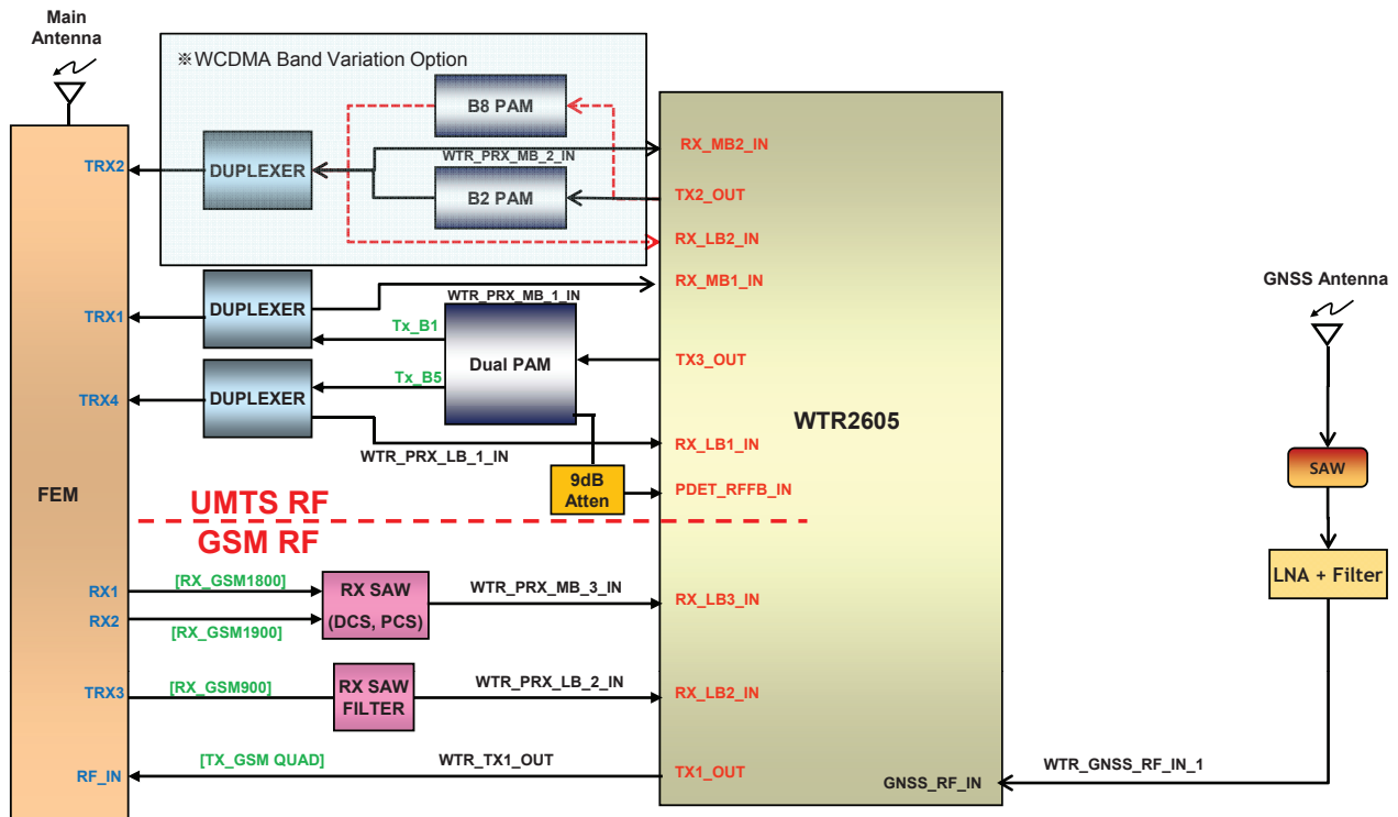
[D370] RF Block Diagram
