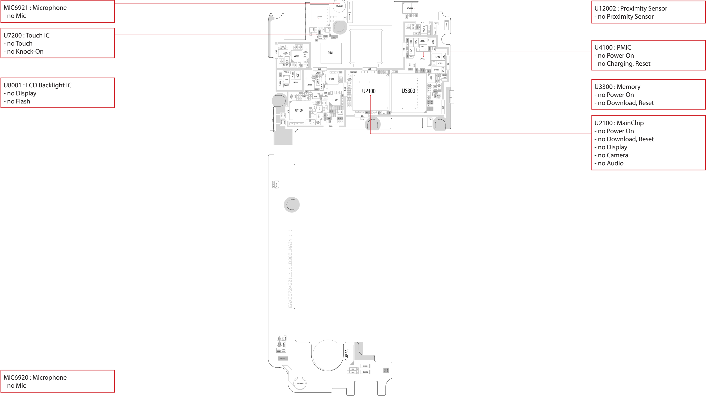
LG-D370_MAIN_EAX65724301_1.0_TOP
