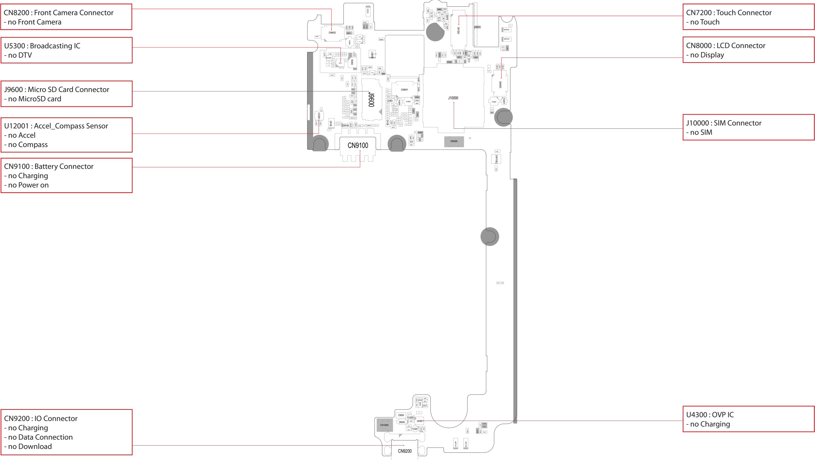
LG-D370_MAIN_EAX65724301_1.0_BOT
