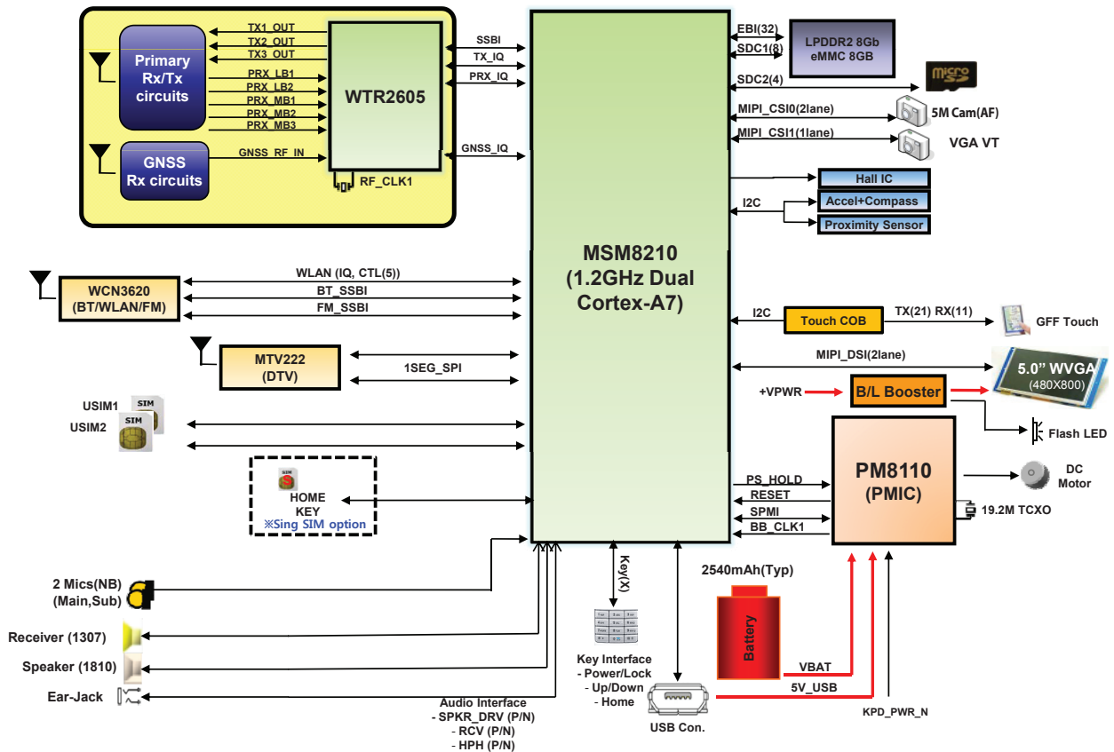
[D370] Total Block Diagram
