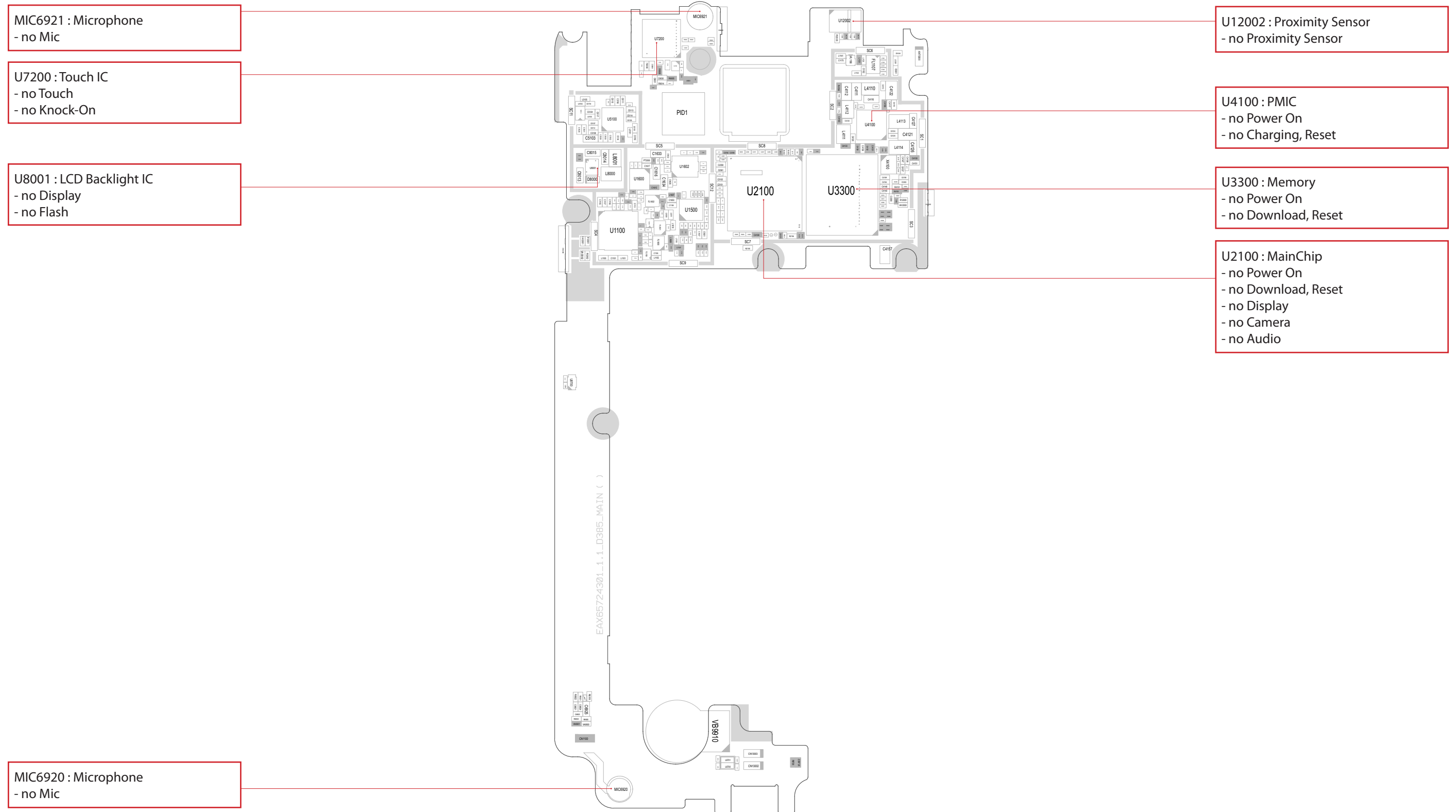
LG-D370TR_MAIN_EAX65724301_1.0_TOP
