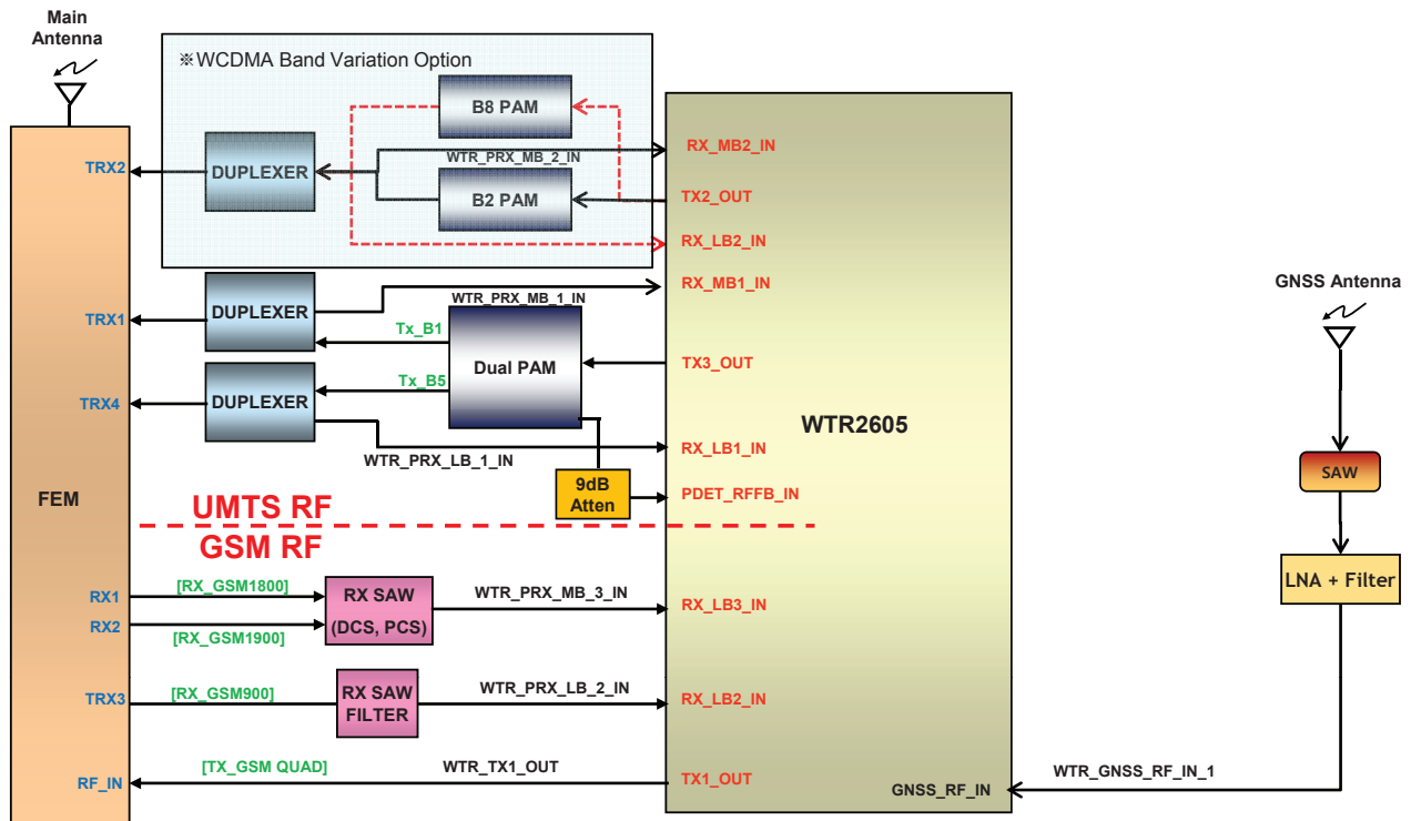
[D370TR] RF Block Diagram
