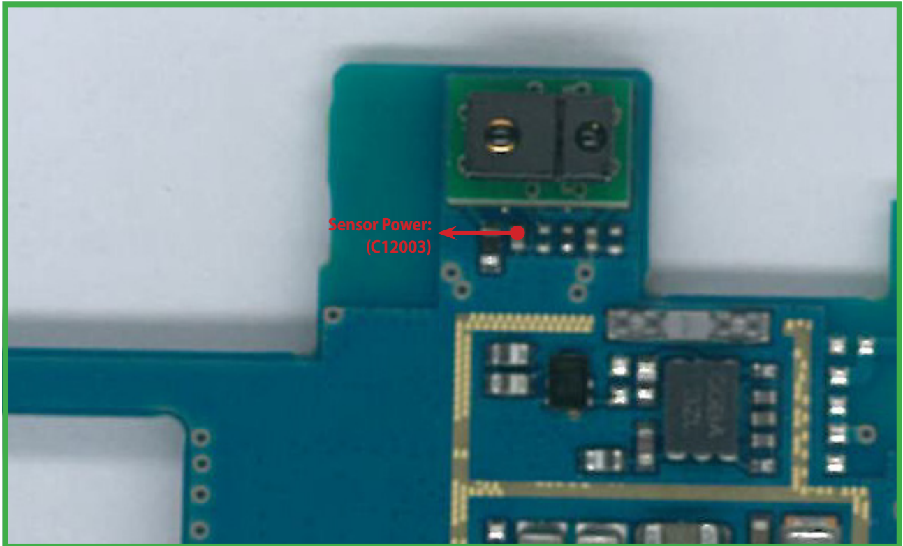
<Main Top>
