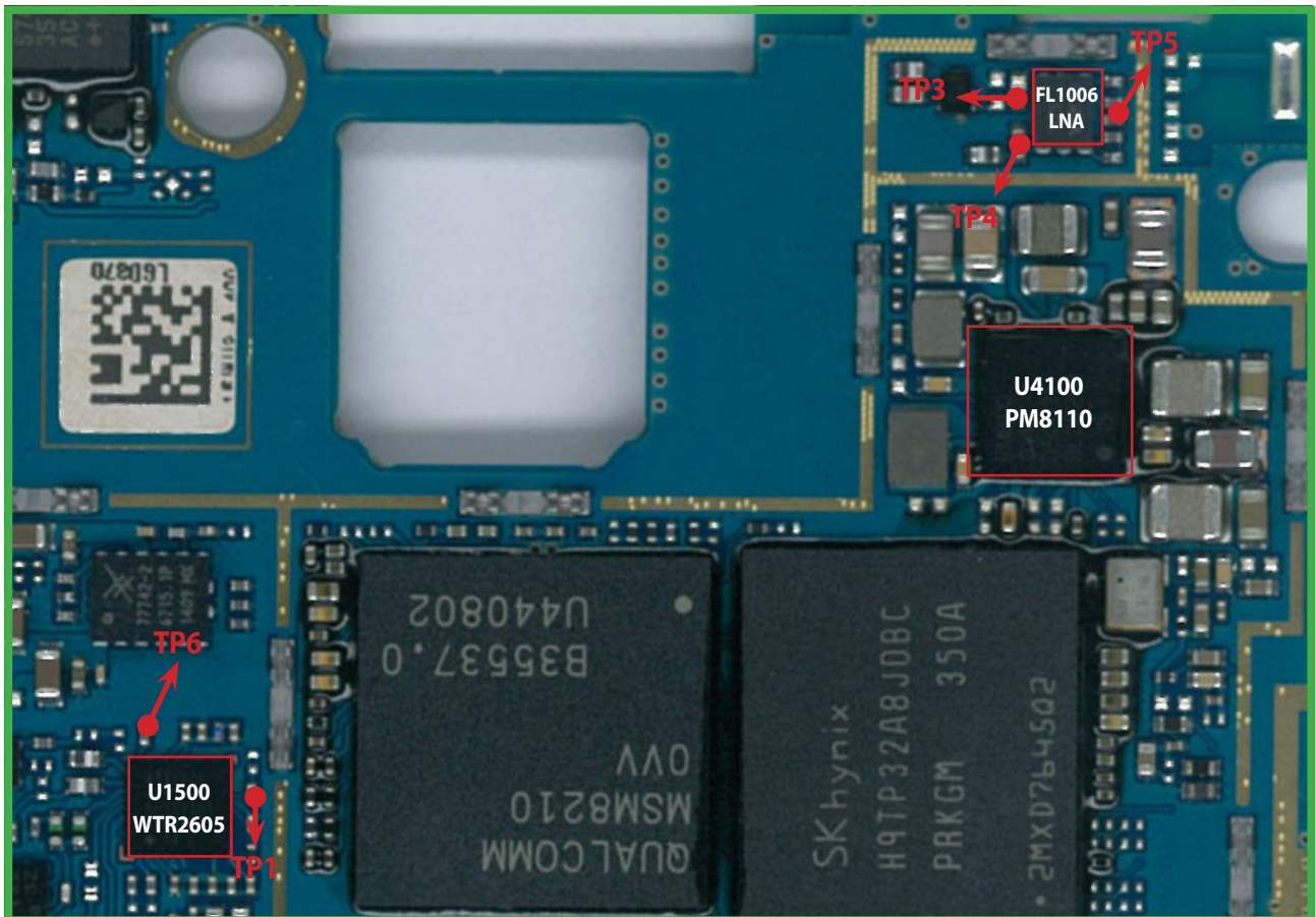
<Main Top>
