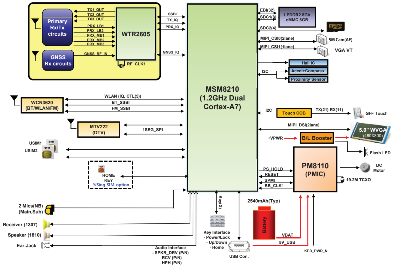
[D370TR] Total Block Diagram
