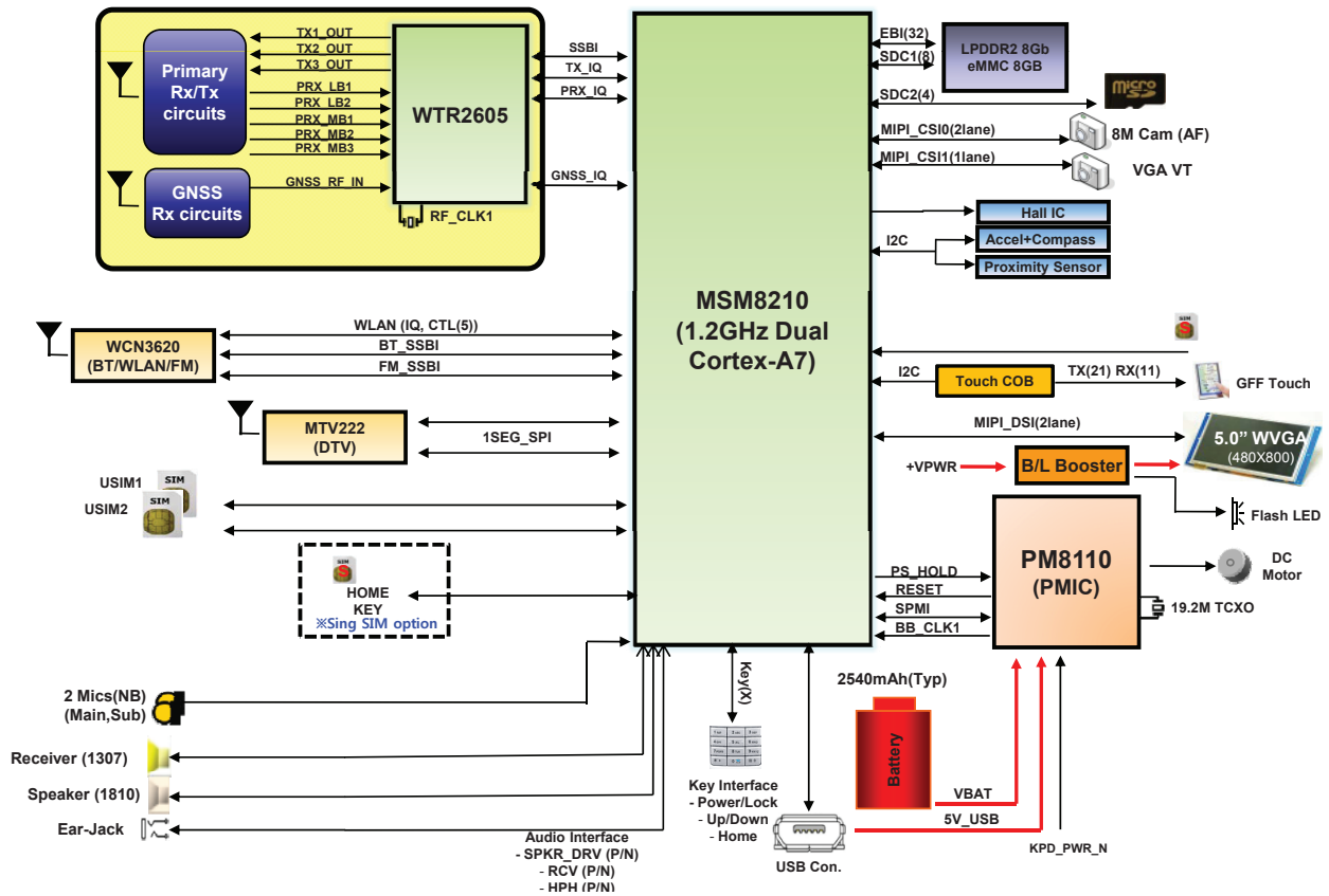
[D373] Total Block Diagram
