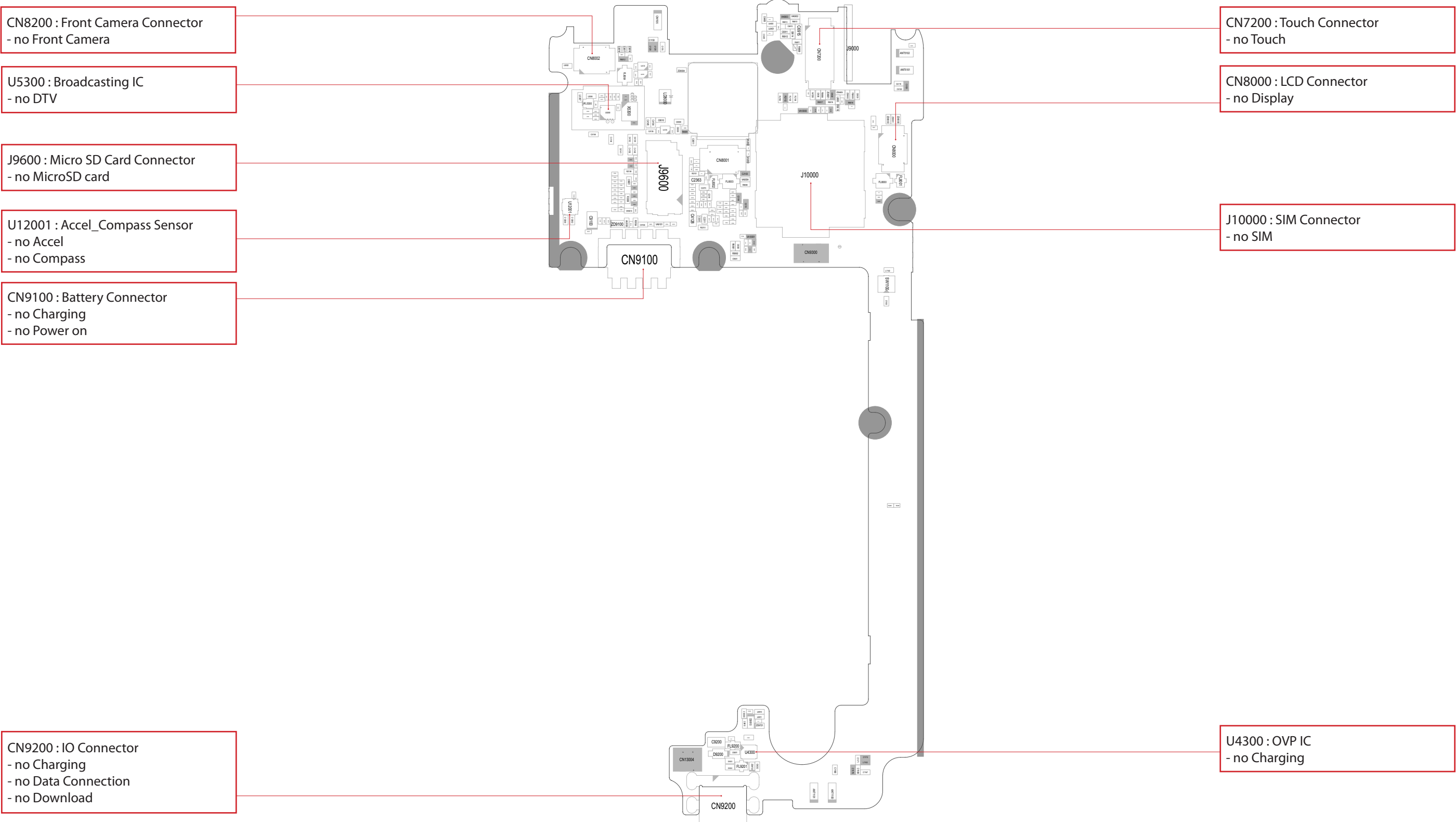
LG-D373_MAIN_EAX65724301_1.0_BOT
