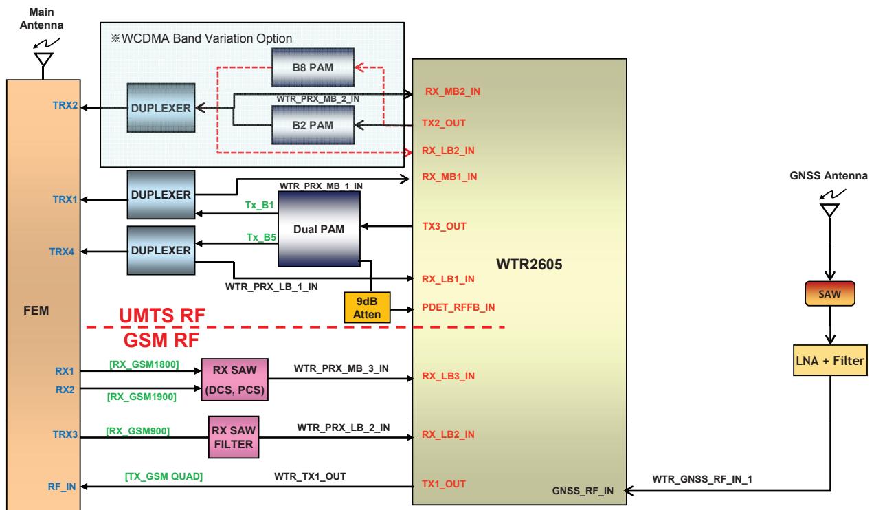
[D373] RF Block Diagram
