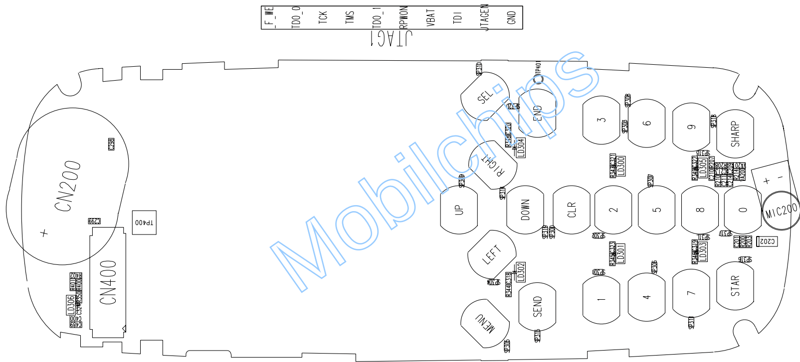
Figure 8-1 B2000 TOP SIDE PCB LAYOUT
