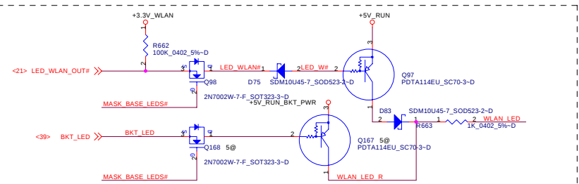
WLAN&BKT LED solution for Blue LED
