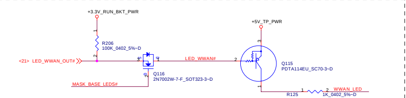
WWAN LED solution for Blue LED
