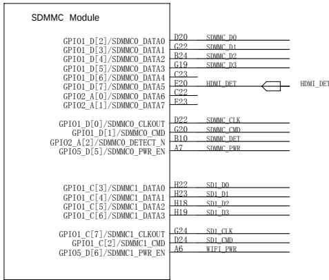
U1-F RK2918 BG512
