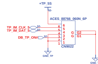
Connect to Mainboard's TP connector
