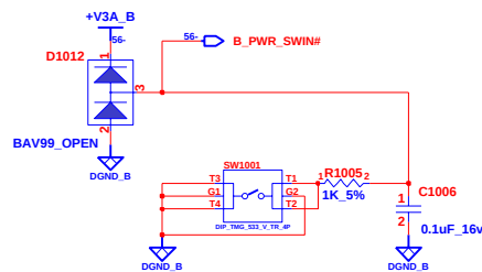
PWR SWITCH
