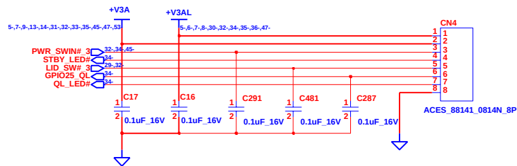
SWITCH Board & LED Board CONN
