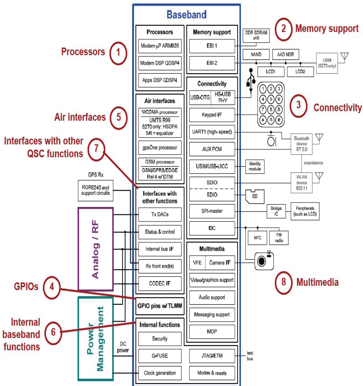
Figure 3.1 QSC6270(3G disable) Base band block
