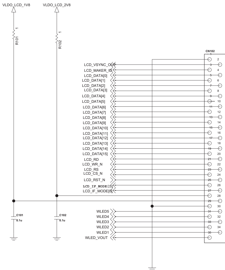
Figure 3.1.7.2.2 The LCD interface of C320i
