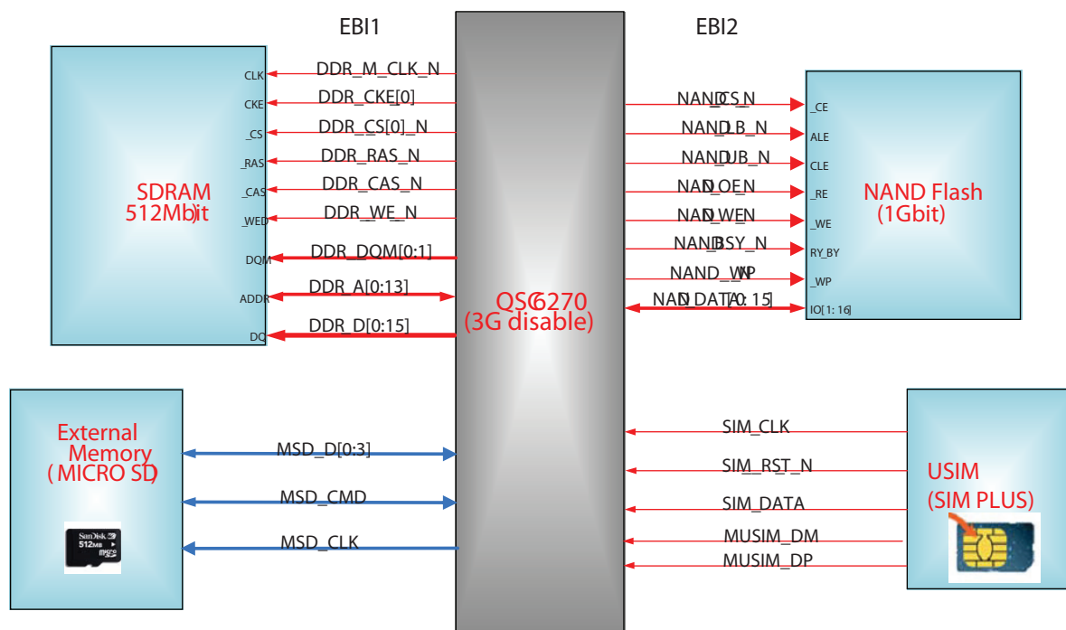
Figure 3.1.2.1 The memory control blocks of C320i
