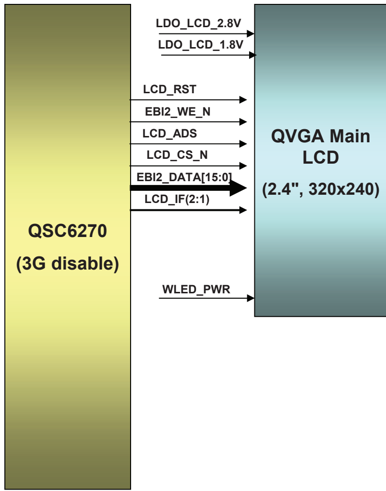
Figure 3.1.2.2 The LCD interfaces of C320i
