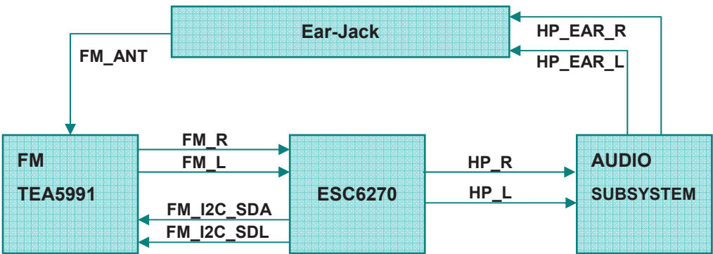
[Figure3.7.2] FM Radio system architecture
