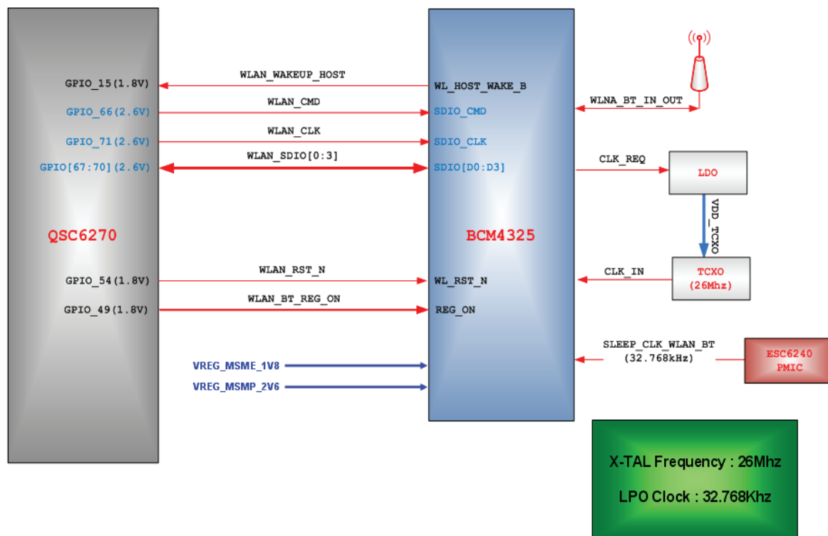
[Figure 1.1] WLAN system architecture
