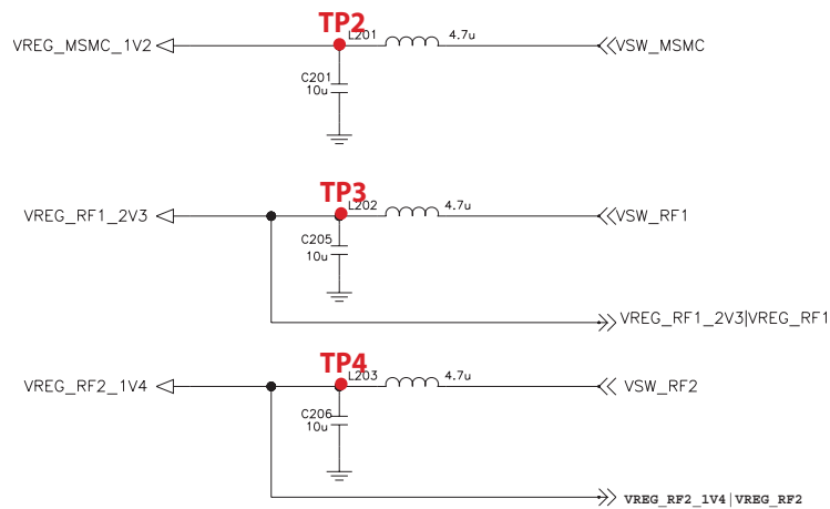
SMPS Circuit
