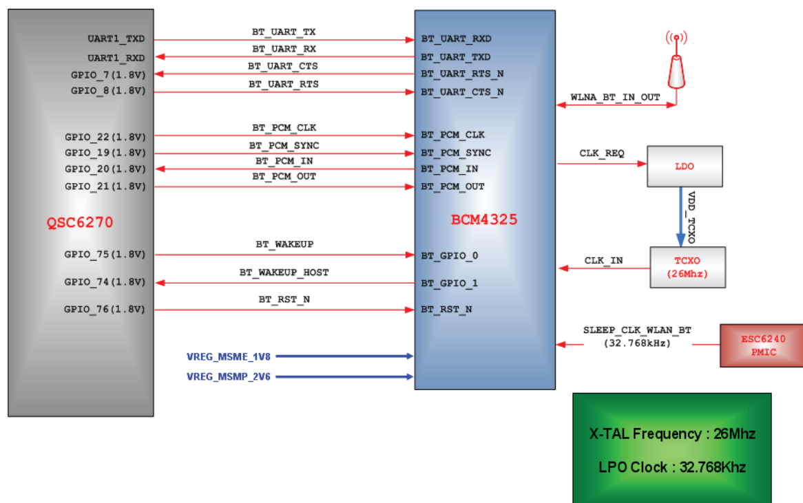
[Figure 1.2] Bluetooth system architecture
