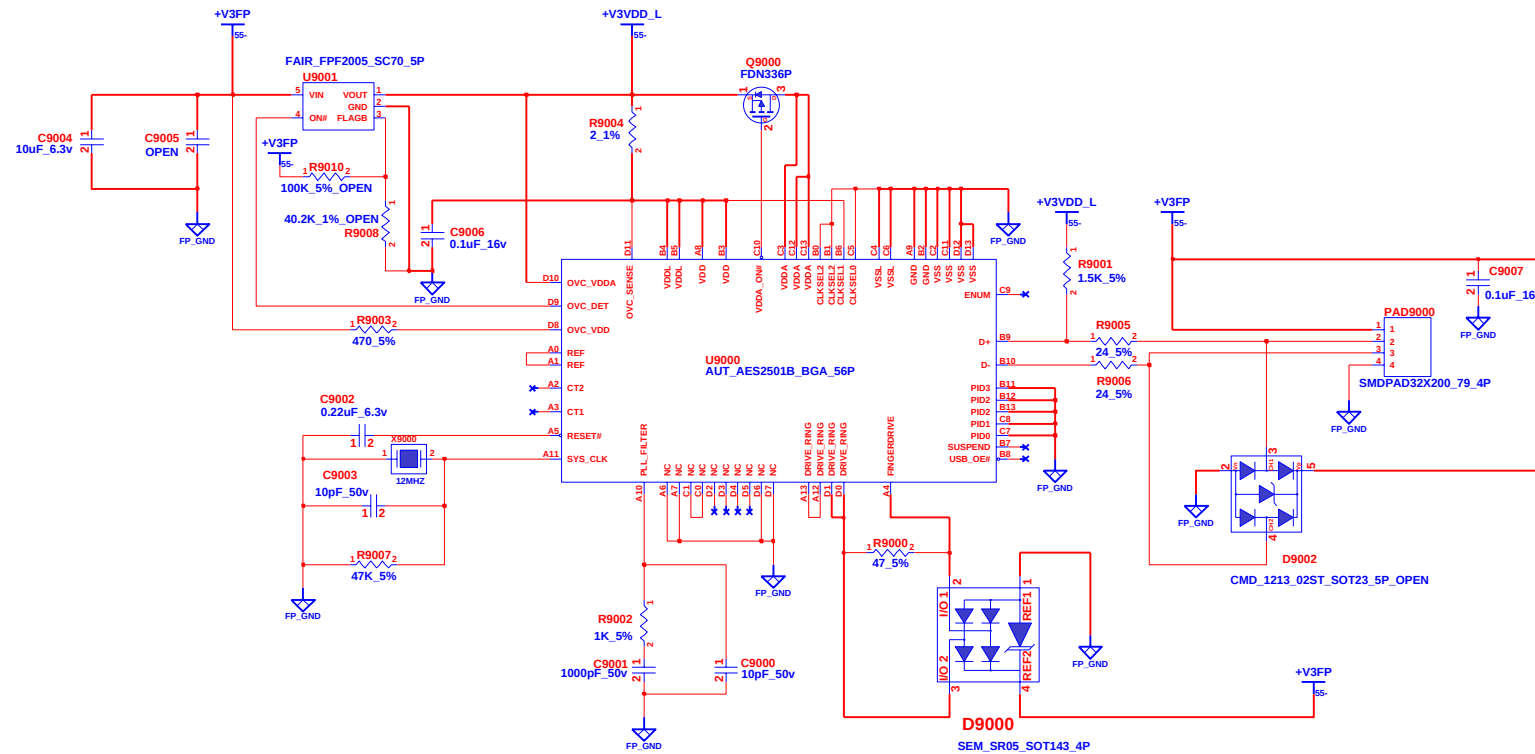
Finger Print Reader DB (Same as DAVOS30 FPR circuit.)
