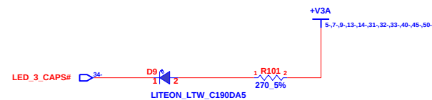
CAP LED
