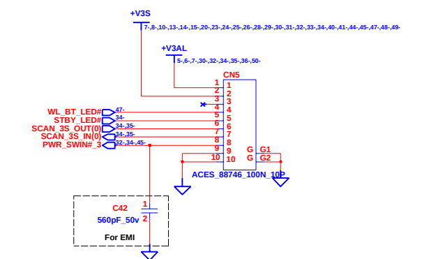
SWITCH DAUGHTER CONNECTOR
