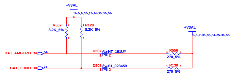
BATTERY-CHARGE LED
