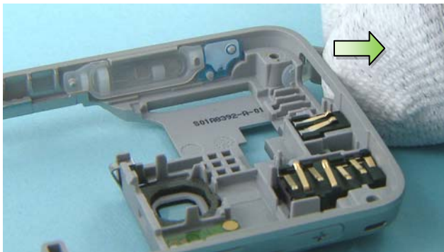
23) Carefully pull out the USB PLUG.
