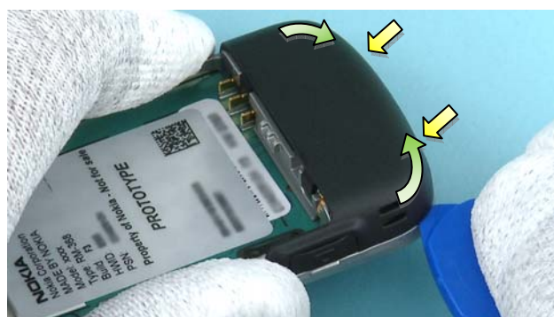
16) To detach the ANTENNA COVER ASSEMBLY, detach the two clips by sliding the SRT-6 along the bottom edge of the cover.
