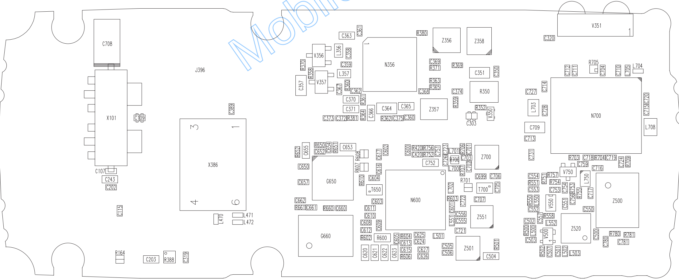
Layout Diagram of LA5 – Bottom (Version 17)
