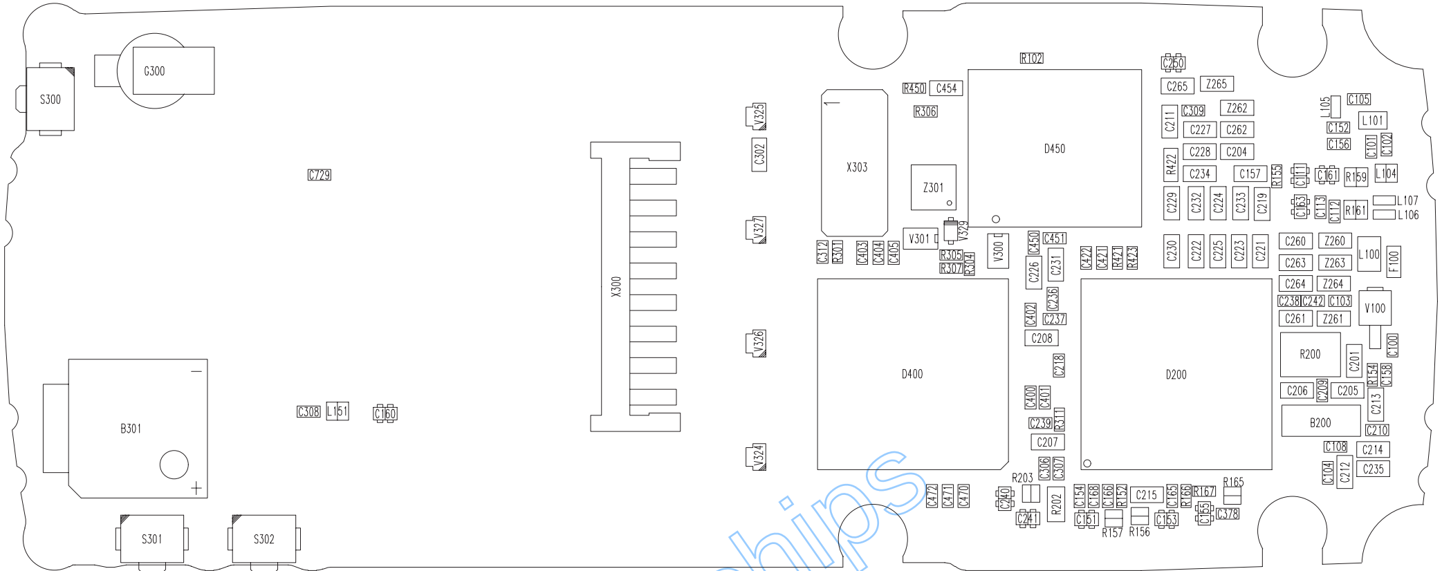
Layout Diagram of LA5 – Bottom (Version 17)
