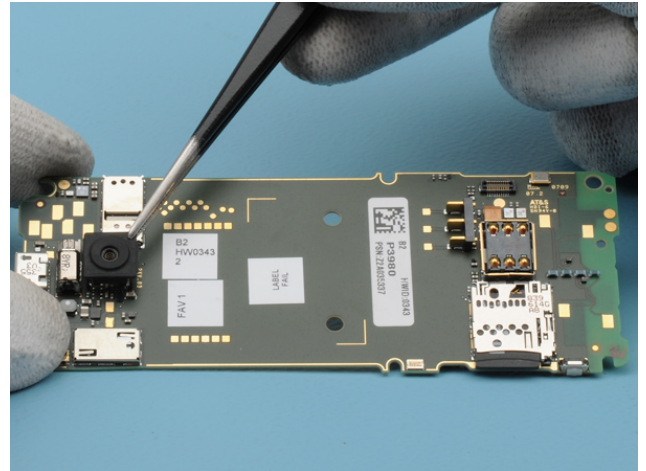
19) Use the tweezers to release the CAMERA BOOT.
