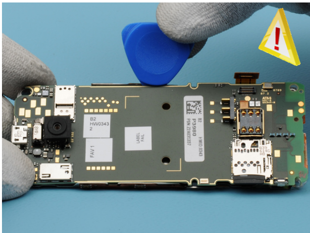
14) Use the SRT-6 to carefully lift the LIGHT SWAP PWB from the UI SHIELD ASSEMBLY.
