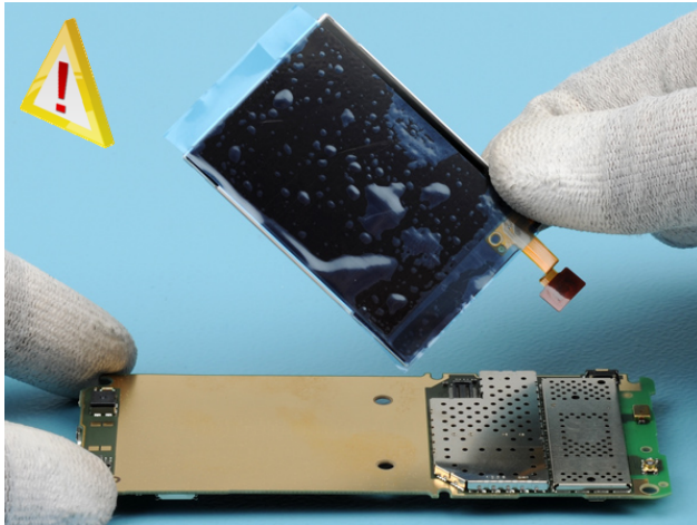
18) Carefully remove the LCD.
