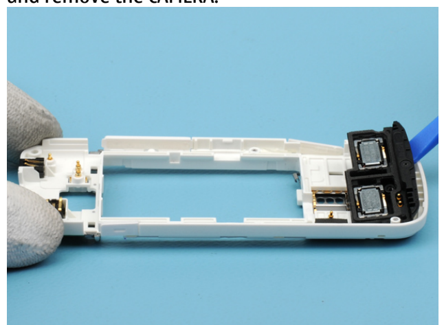
23) Use the SS-93 tool to release the ANTENNA ASSY.
