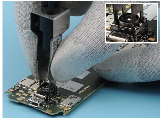
21) Use the SS-88 tool to release the CAMERA. Lift and remove the CAMERA.
