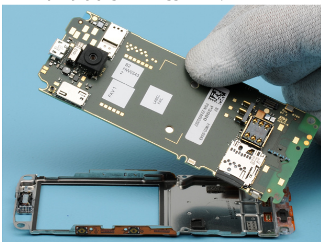
16) Separate the UI SHIELD ASSEMBLY and the LIGHT SWAP PWB.
