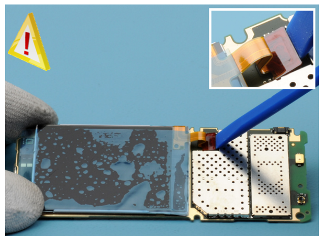
17) Use the SS-93 tool to carefully open the LCD CONNECTOR.
