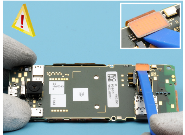
13) Use the SS-93 tool and carefully release the UI CONNECTOR.
