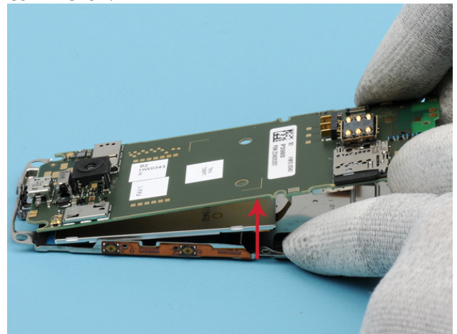
15) Lift the LIGHT SWAP PWB as shown.
