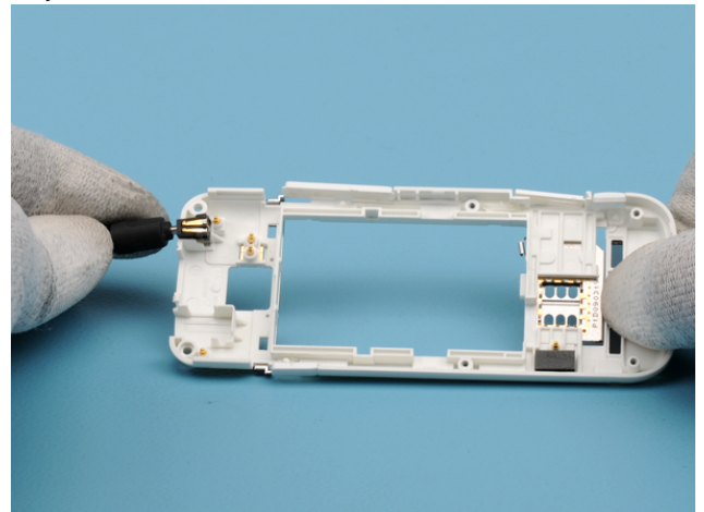
27) Use the charger plug to release the CONN CHR DIA 2.0MM COMPRESS.
